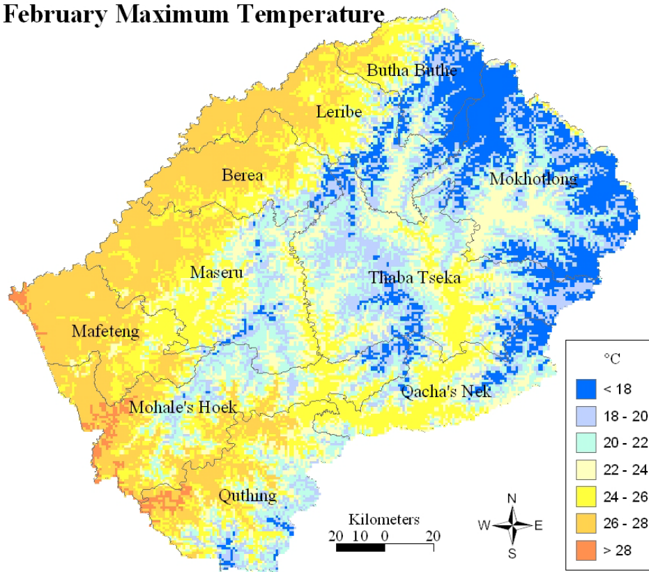
Fig 4.8 Maps of mean monthly maximum temperature for January and February
