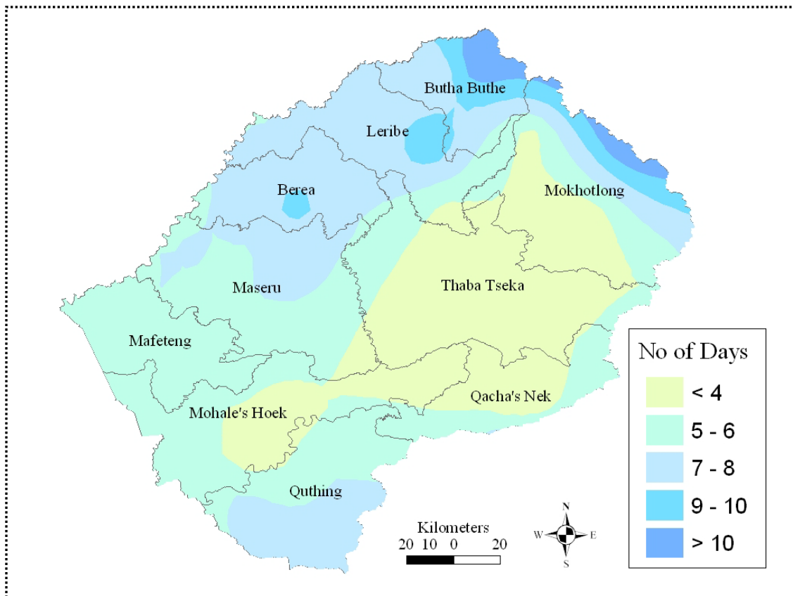
Fig 5.11 Map of average number of days with daily rainfall \geq 25\text{mm} per year for Lesotho
