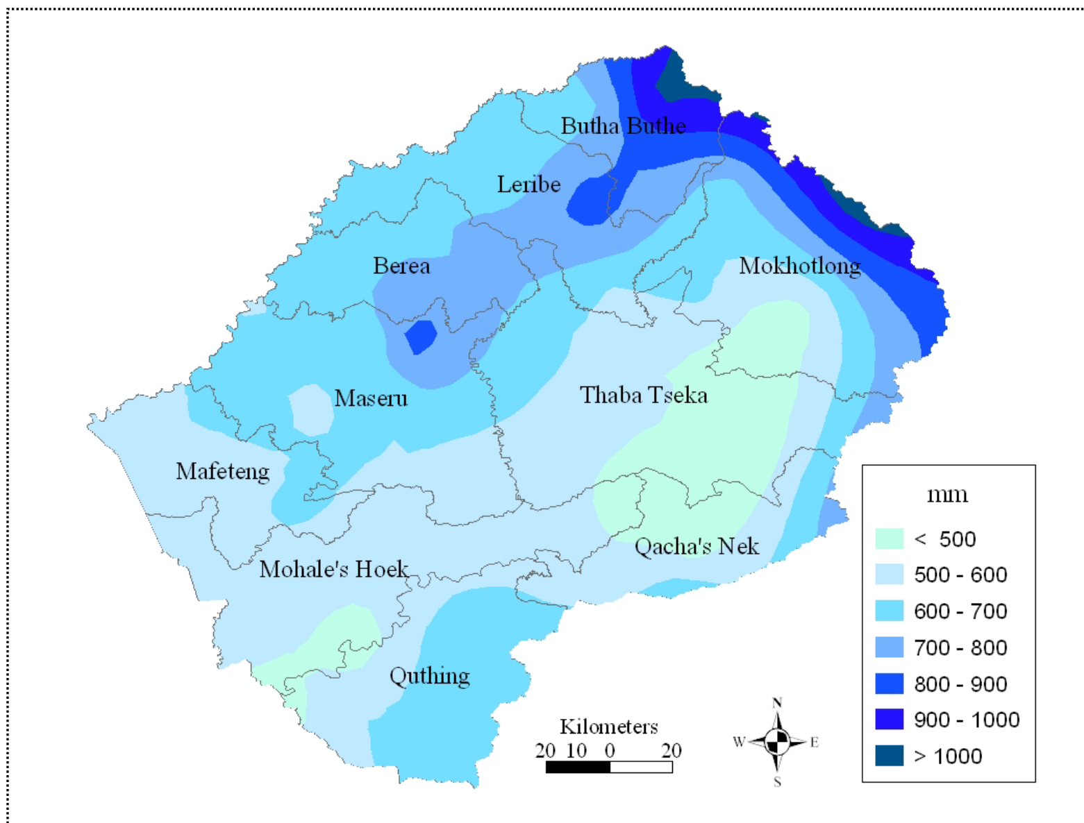
Fig 5.9 Average wet season (October to April) precipitation map of Lesotho obtained using kriging interpolation method (Data from Lesotho meteorological services)
