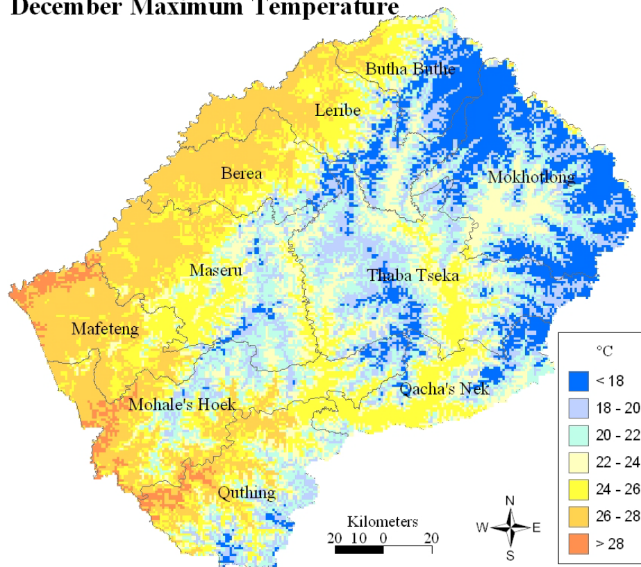
Fig 4.13 Maps of mean monthly maximum temperature for November and December
