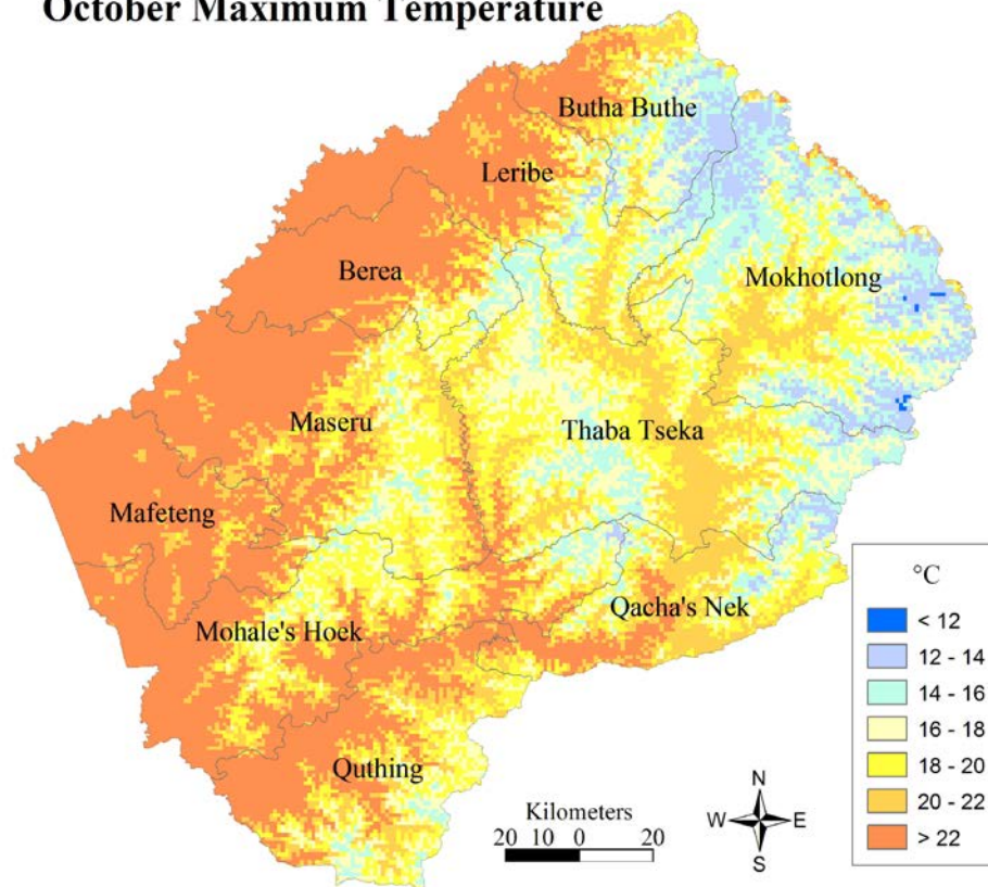
Fig 4.12 Maps of mean monthly maximum temperature for September and October
