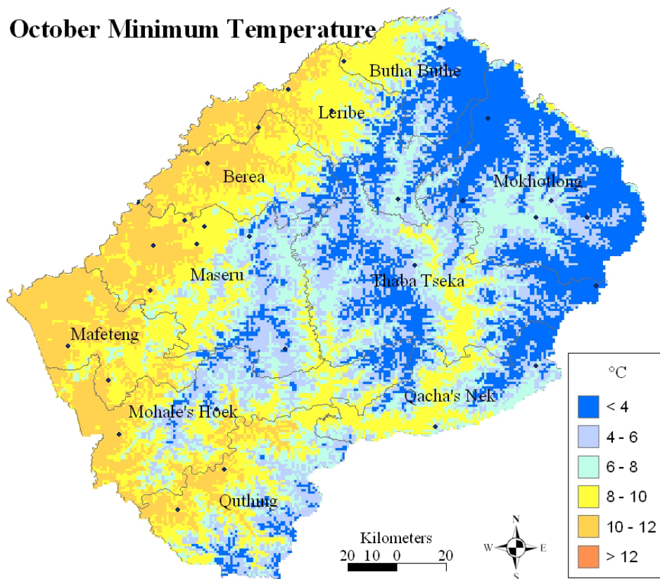
Fig 4.6 Maps of mean monthly minimum temperature for September and October
