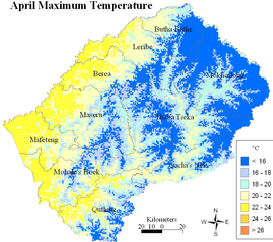
Fig 4.9 Maps of mean monthly maximum temperature for March and April
