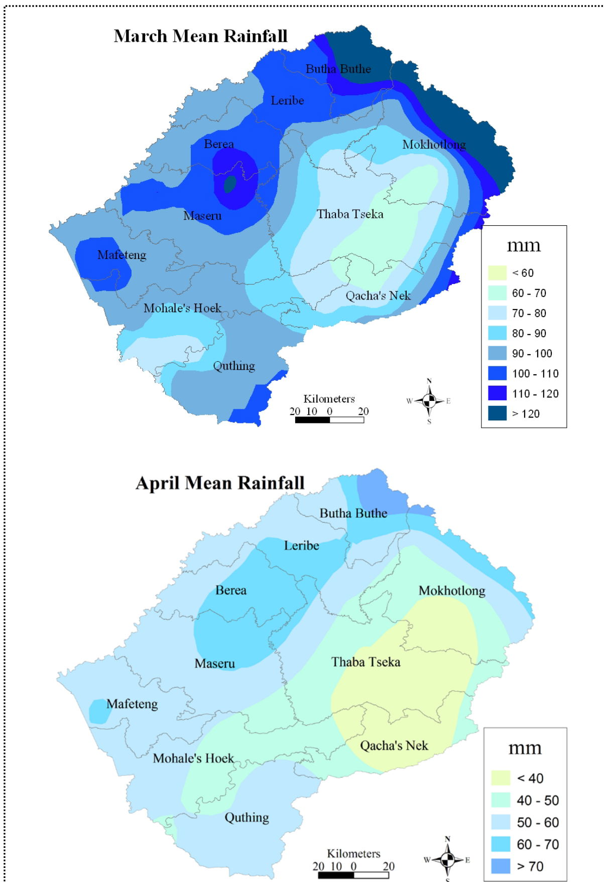
Fig 5.3 Maps of monthly rainfall for March and April
