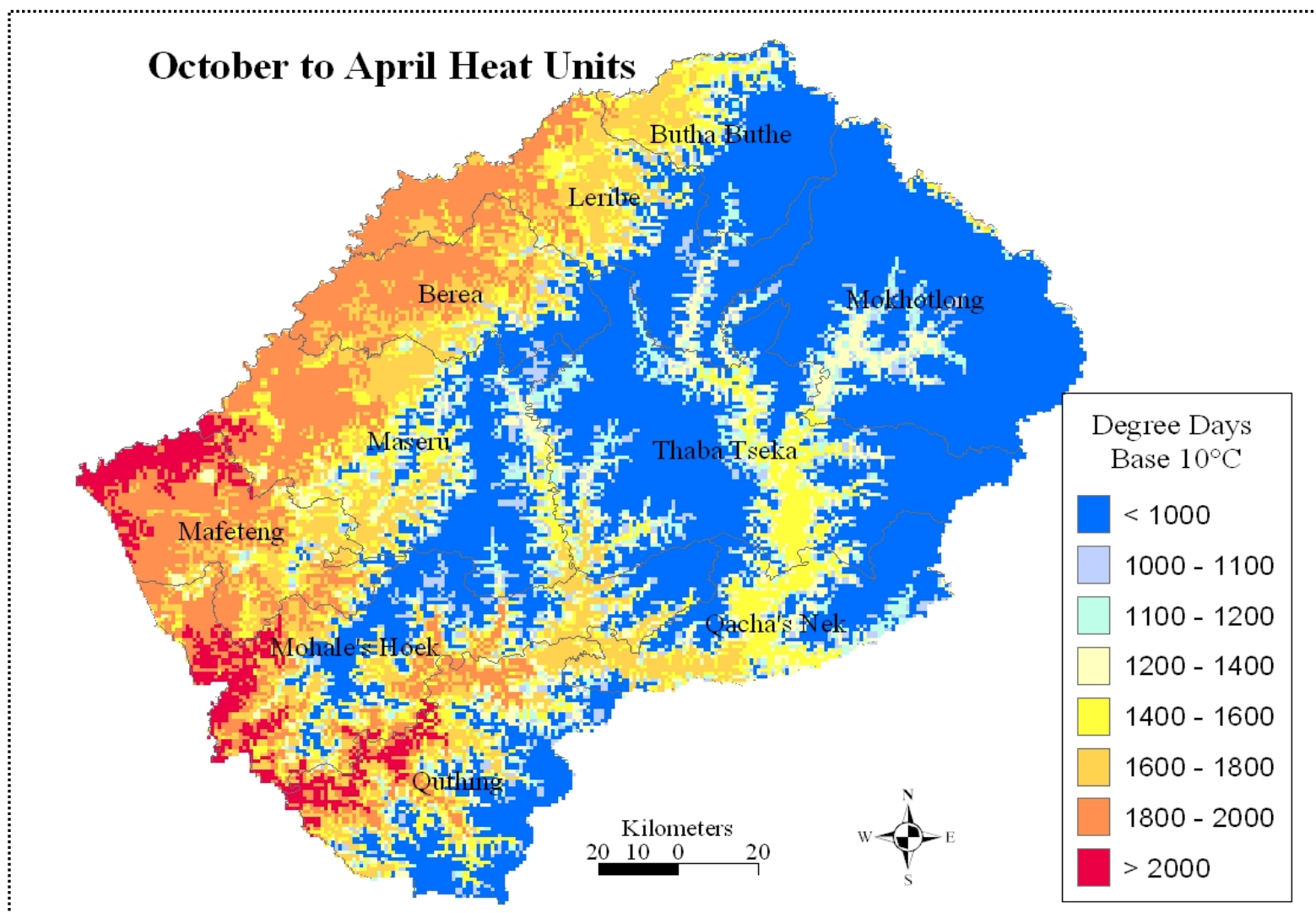
Fig 4.20 Map of seasonal (October to April) heat units for the country of Lesotho using the equation GDD = \left[ \frac{(T_{MAX} + T_{MIN})}{2} \right] - T_{BASE} Where
