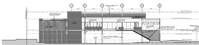
11 LIBRARY SOUTH ELEVATION Scale 1:100
