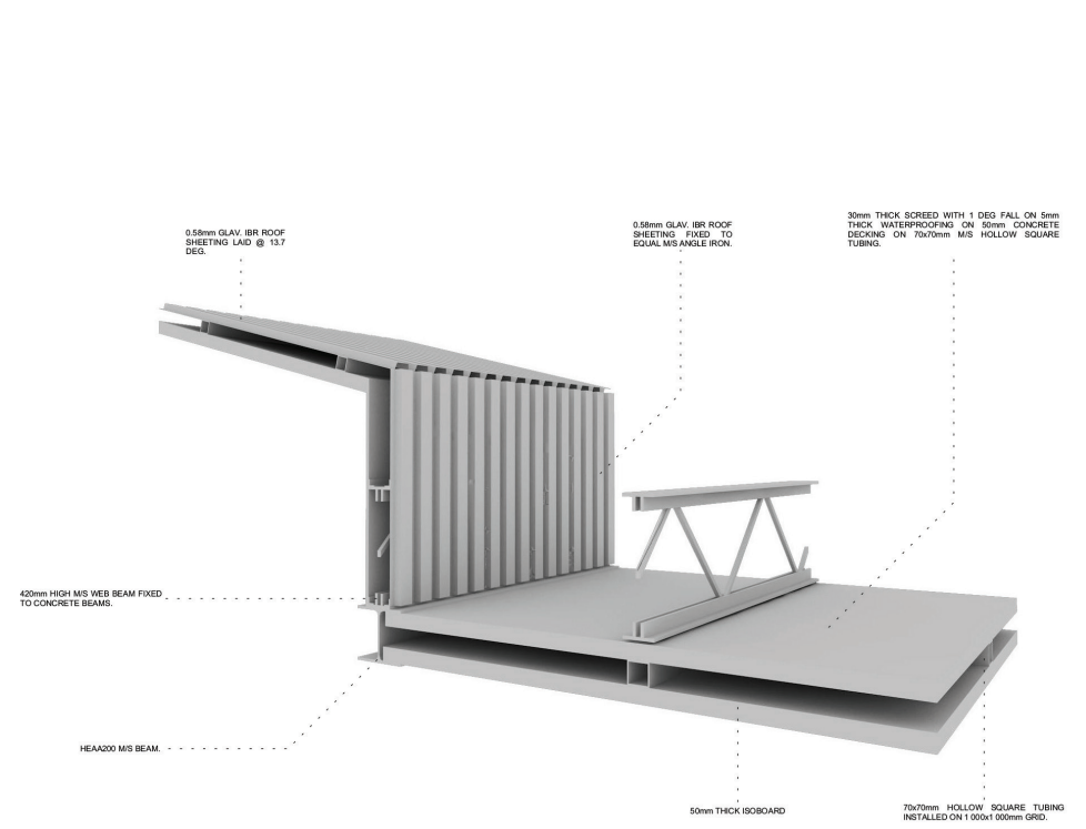
2 — DETAIL 3 - VIEW 2
