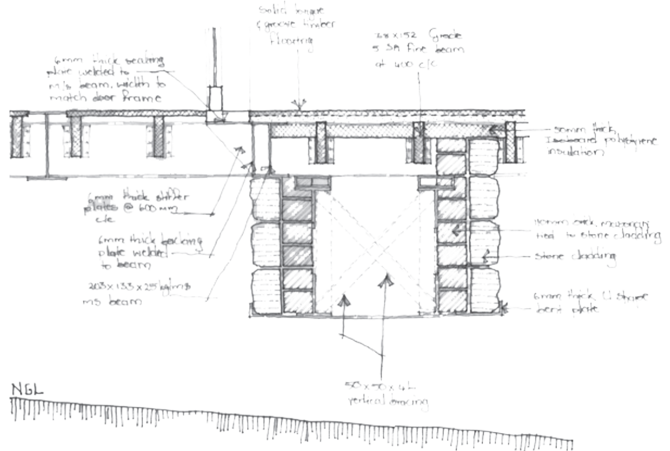
Figure 141: Cross section (left) & floating wall detail (right) (derived from Louw, 2014)
