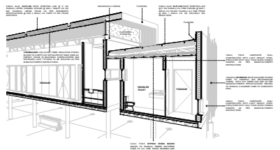
5 PART PERSPECTIVE SECTION F.F Scale 1:50
