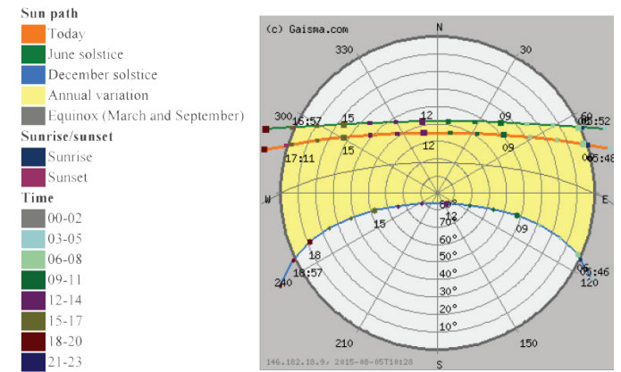
Figure 131: Sun path diagram (Tukiainen, [n.d.]: Online)
