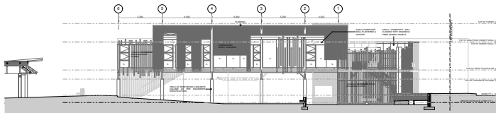
10 LIBRARY NORTH ELEVATION Scale 1:100
