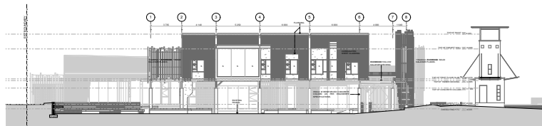
2 GIPF MANAGEMENT SOUTH ELEVATION Scale 1:100
