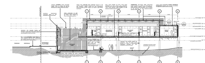
12 SECTION G.G Scale 1:100
