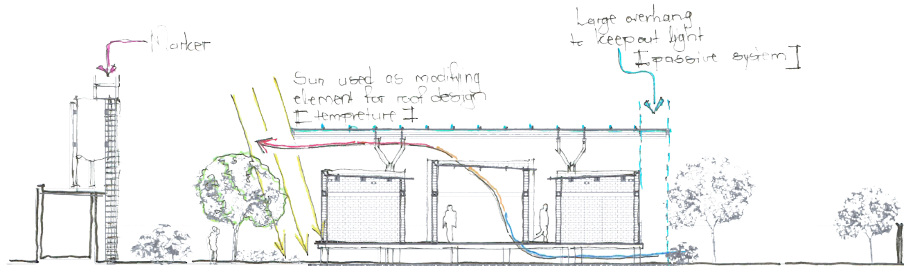
Figure 81: Simple passive cooling systems 1 (derived from Fernandez-Galiano, 2011)
