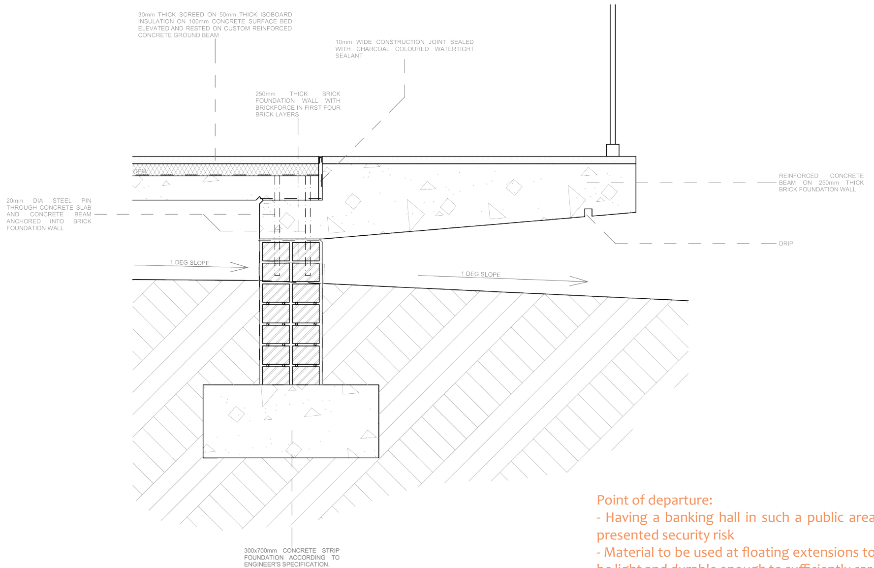
2 GROUND TO FLOOR DETAIL_SUSPENDED SLAB
