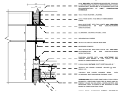
13 DETAIL 1 Scale 1:50
