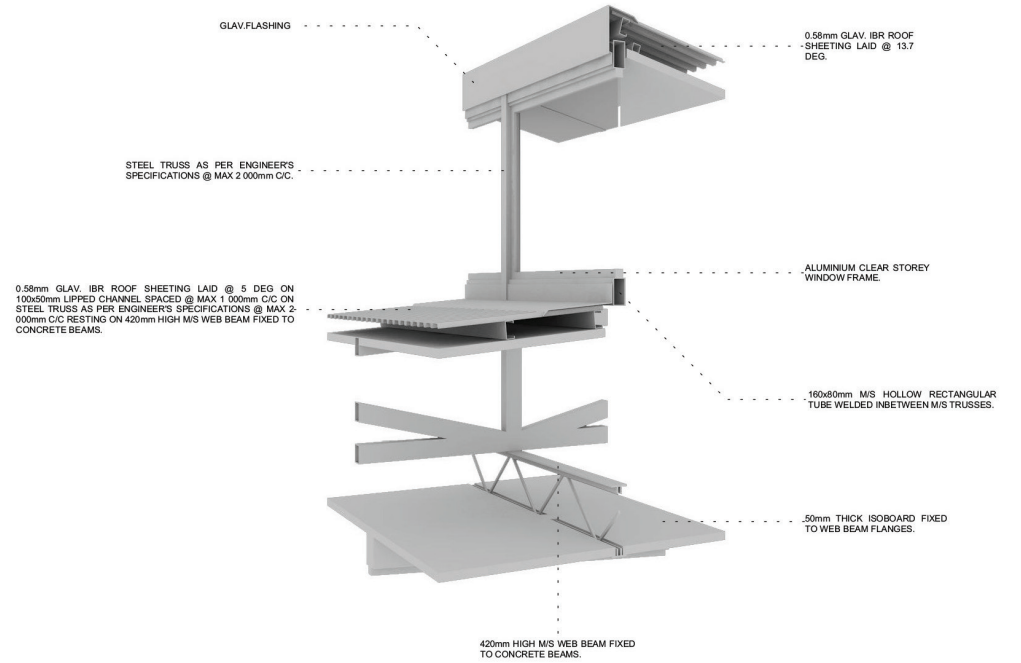
2 DETAIL 1 - VIEW 2
