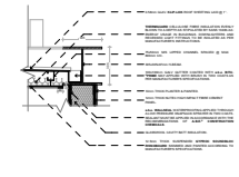
14 DETAIL 2 Scale 1:50
