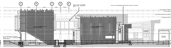
9 EAST ELEVATION - PART 2 Scale 1:100
