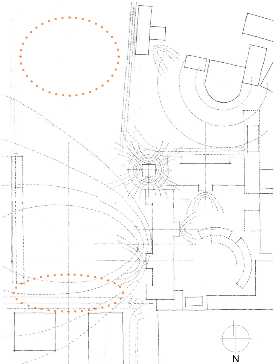
Figure 94: Radiance study as per Von Meiss' principles
