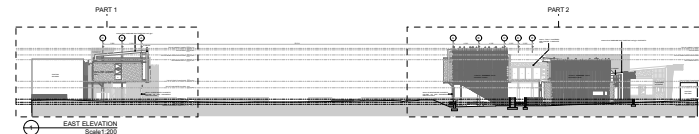
6 EAST ELEVATION - PART 1 Scale 1:100
