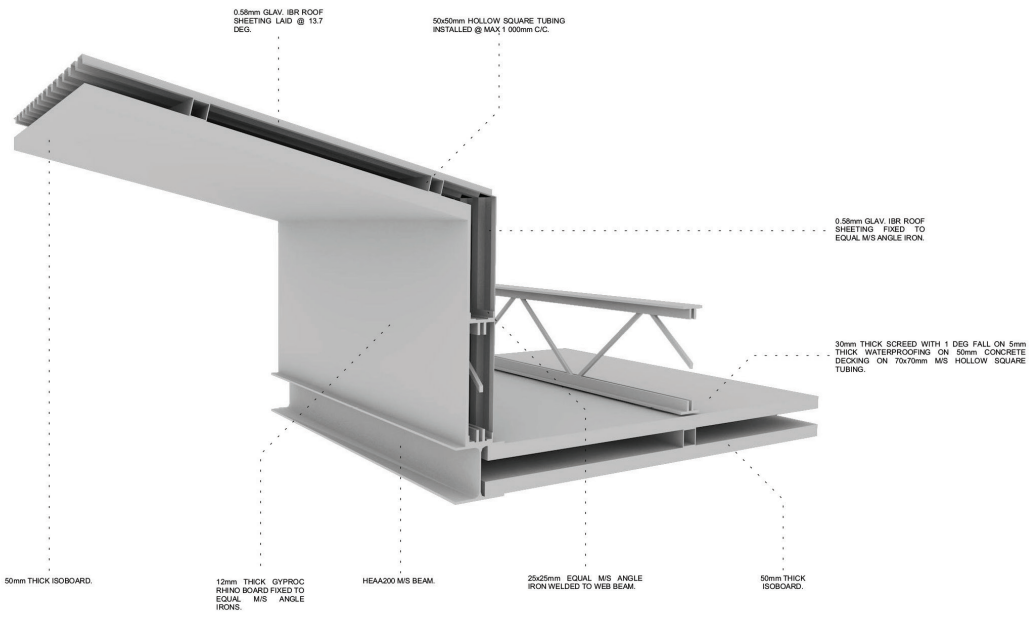
1 — DETAIL 3 - VIEW 1
