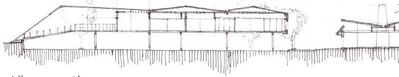
Library section
