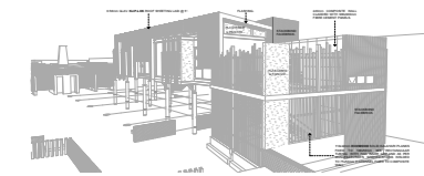
15 LIBRARY ENTRANCE PERSPECTIVE Scale 1:50
