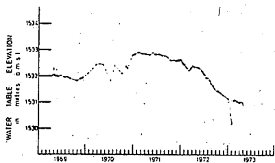
BOREHOLE W 522
