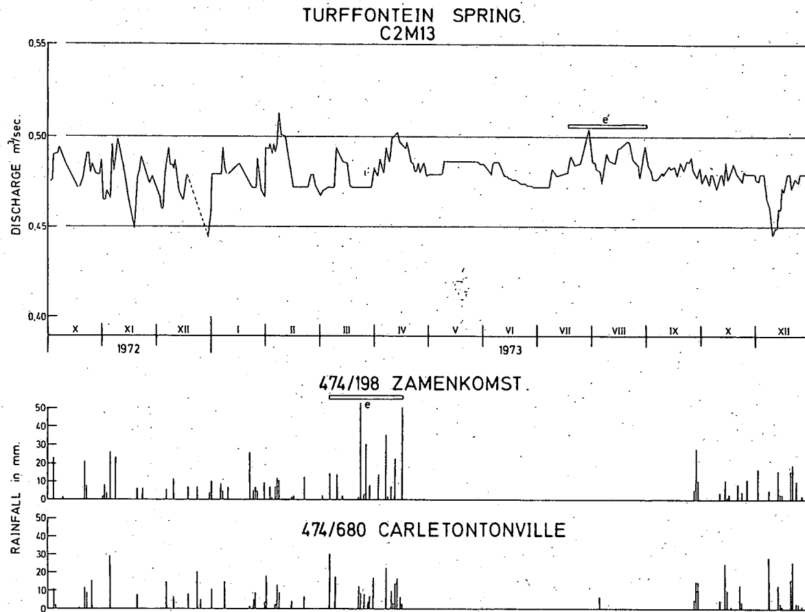
Fig.10.3 Daily discharge against daily rainfall. A four month phase difference observed between a rainy episode and its manifestation in the discharge
