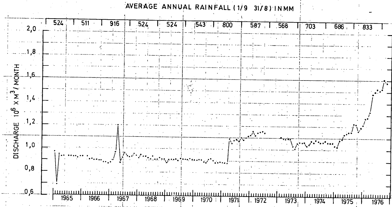
Fig.9.4 MONTHLY DISCHARGE AT MALONY'S SPRING
