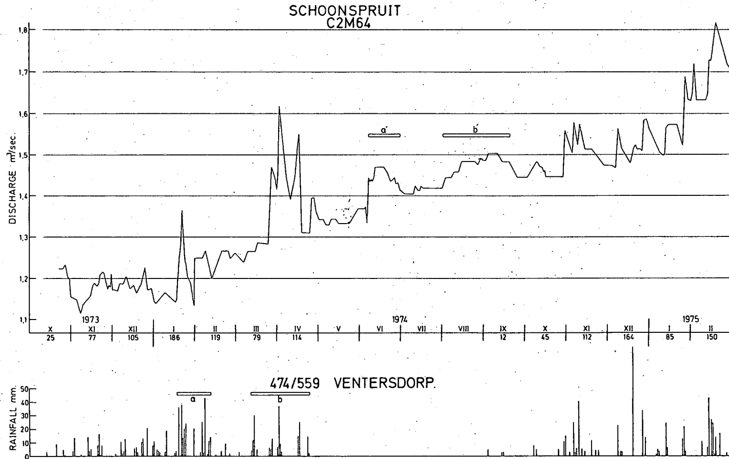
Fig.10.4 Daily discharge against daily rainfall. A six month phase difference observed between a rainy episode and its manifestation in the discharge.
