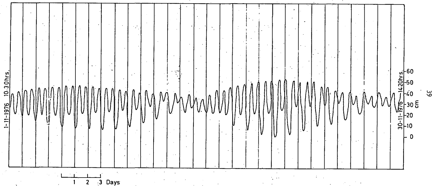
Fig. 56 AUTOMATIC WATER LEVEL RECORDING IN BOREHOLE GB16 ILLUSTRATING TIDAL EFFECTS IN PARTS OF THE AQUIFER
