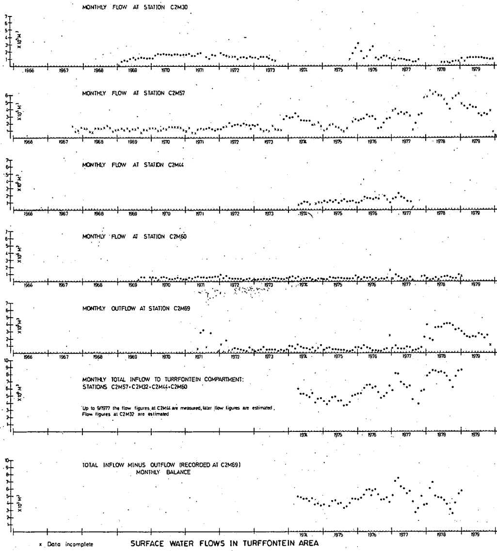
SURFACE WATER FLOWS IN TURFFONTEIN AREA Fig. 9.1
