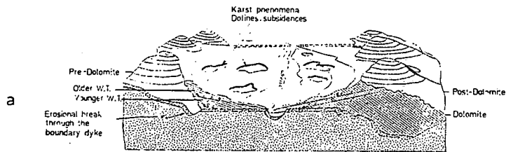
Block diagram showing an early phase of karstification. The products of karstification form the basal part of the present aquifer. Depth of karstification was regulated by erosion of the boundary dykes.
