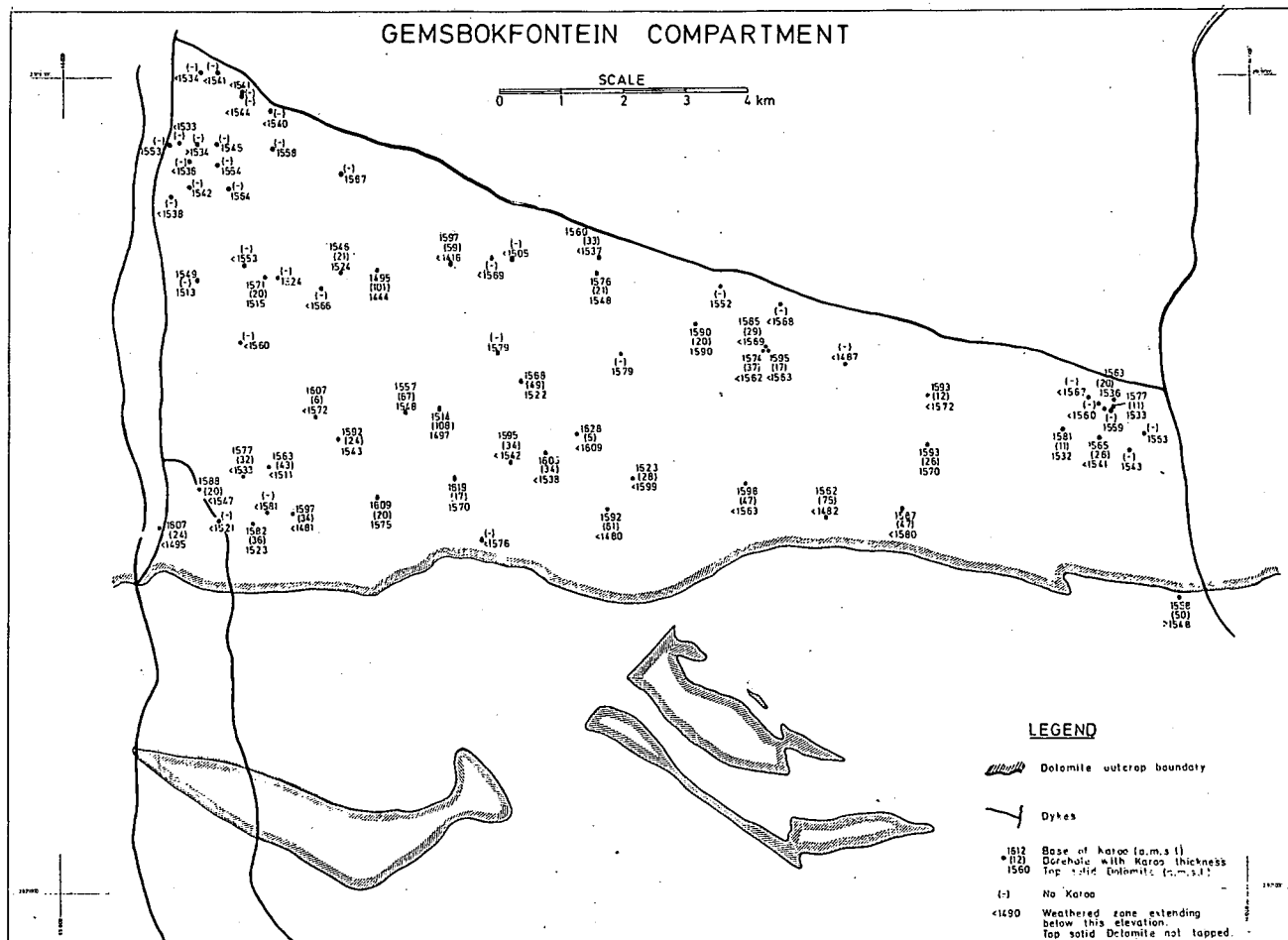
FIG. 6.28 BASE OF KAROO A.M.S.L
