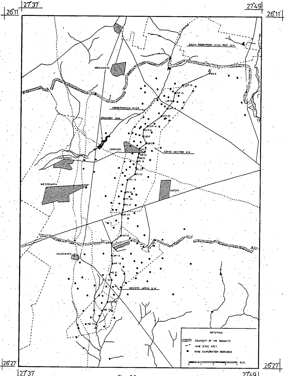
Fig. 3.2 KEY MAP FOR CROSS-SECTION A-A'
