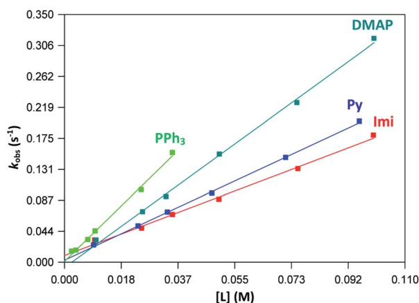
Fig. 7 Plot of k_{\text{obs}} vs. ligand concentration for each ligand at 25 °C indicating linear kinetic traces for the concentration ranges of 0.01–0.1 M.
