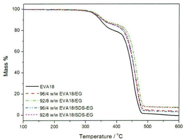
Figure 2.8 TGA curves of EVA18 and its nanocomposites: EG and SDS modified EG
