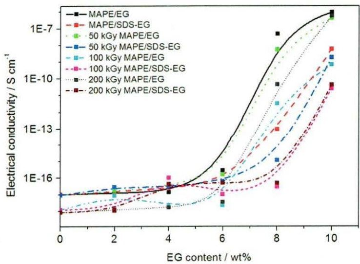
Figure 5.5 Electrical conductivities of all the investigated samples
