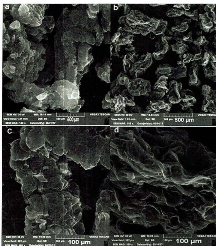
Figure 2.2 SEM micrographs of (a) EG (100 x mag); (b) SDS modified EG (100 x mag); (c) EG (500 x mag); (d) SDS modified EG (500 x mag)
