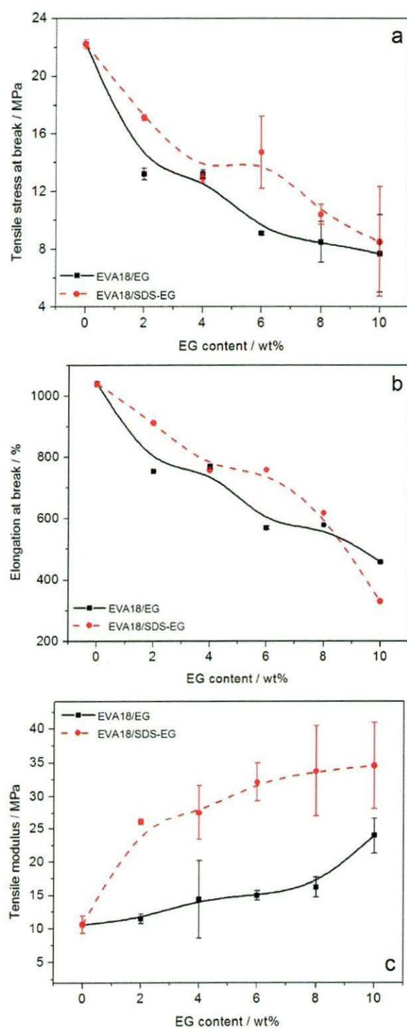
Figure 2.10 Variation of (a) stress at break, (b) elongation at break and (c) tensile modulus of EVA/EG and EVA/SDS-EG samples as a function of filler content
