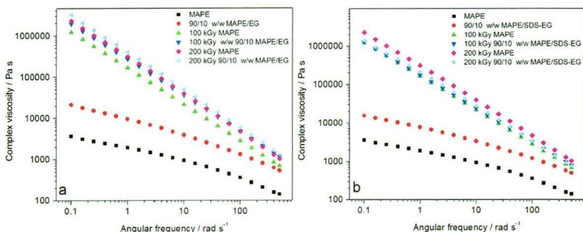
Figure 5.10 Comparison of the complex viscosity at 190 °C of non-irradiated and irradiated (a) MAPE/EG and (b) MAPE/SDS-EG samples as a function of angular frequency
