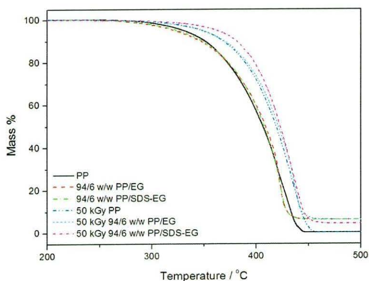
Figure 4.7 TGA curves of the non-irradiated and irradiated samples
