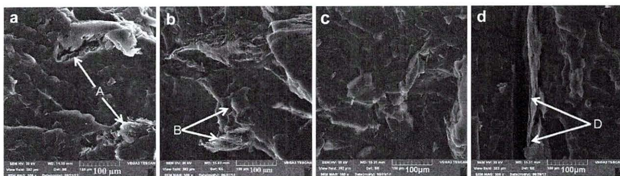
Figure 4.1 SEM micrographs of PP/expanded graphite composites: (a) 98/2 w/w PP/EG; (b) 50 kGy 98/2 w/w PP/EG; (c) 98/2 w/w PP/SDS-EG; (d) 50 kGy 98/2 w/w PP/SDS-EG
