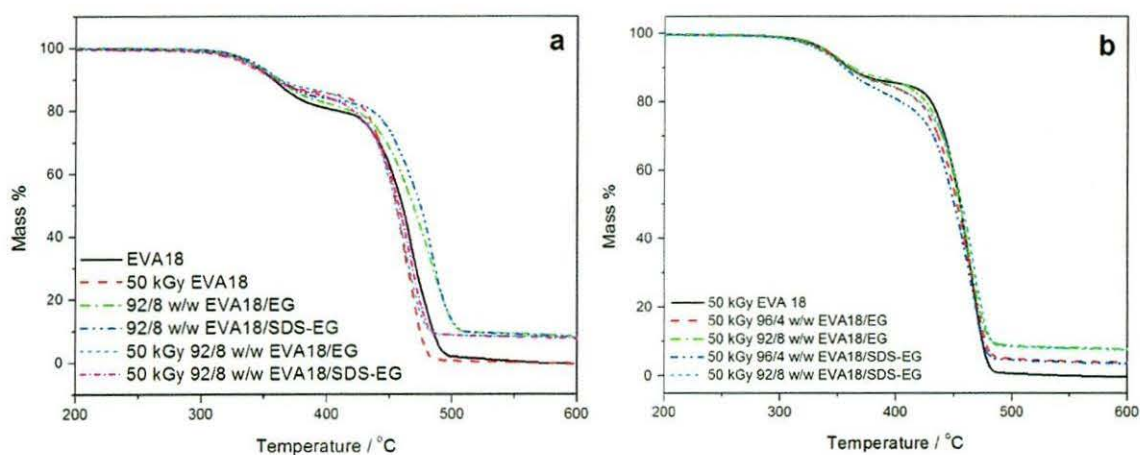
Figure 3.6 TGA curves of non-irradiated and irradiated (a) EVA18/EG and (b) EVA/SDS-EG composites
