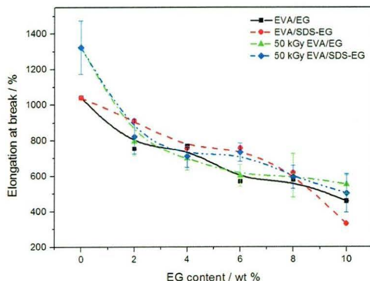
Figure 3.8 Variation of elongation at break of non-irradiated and irradiated EVA/EG and EVA/SDS-EG samples as a function of filler content
