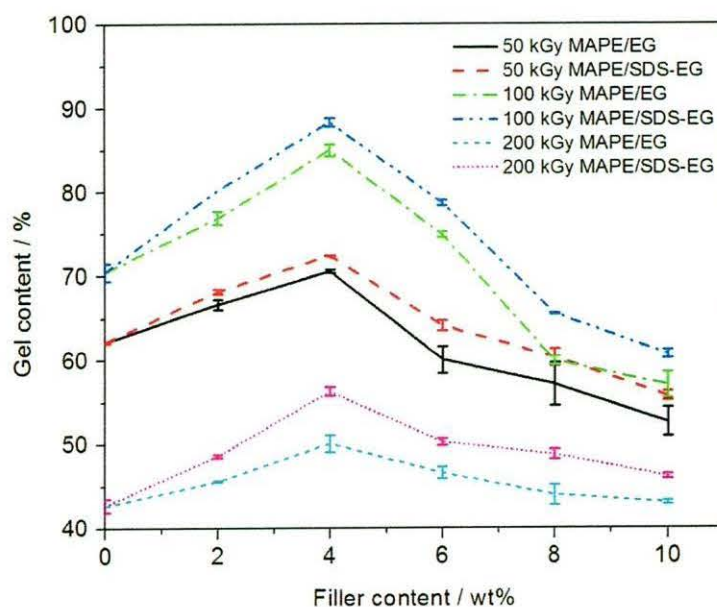
Figure 5.1 Gel content as function of EG content for irradiated samples without and with SDS treatment
