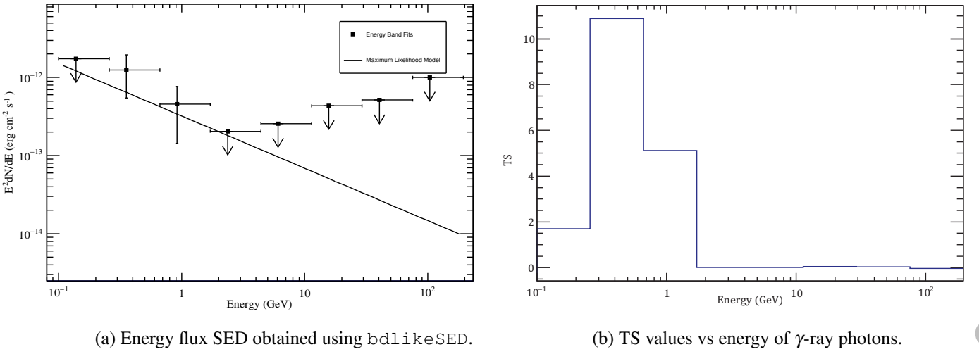
Figure 2: The flux values are 2\sigma upper limits based on a limiting TS < 4 value per bin. Distribution of high energy \gamma -rays are more likely to be detected at lower energies.
