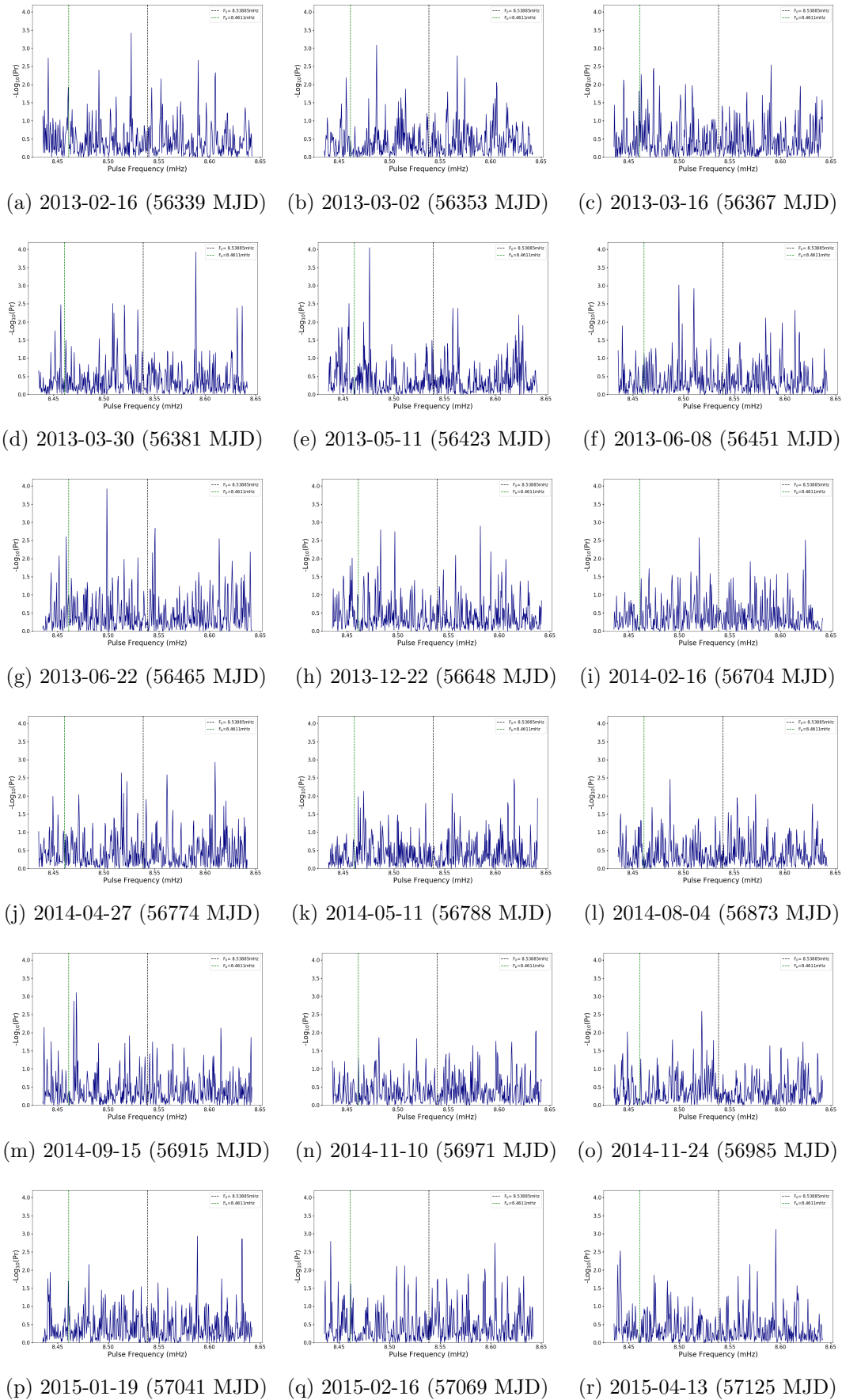
Figure D.5: AR Sco Rayleigh power spectra over selected 2-week periods in the 10-year data set at noise level, continued.
