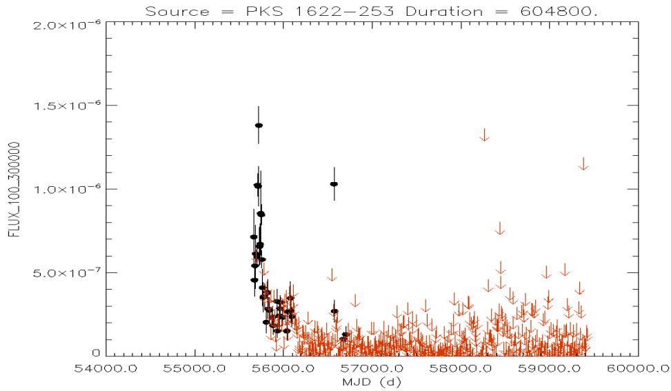
Figure 4.12: Weekly binned light curve of PKS1622-253 that is currently in the Fermi -LAT Monitored Source list. Adopted from https://fermi.gsfc.nasa.gov/ssc/data/access/lat/msl_lc/source/PKS_1622-253 . Accessed 15/10/2021.
