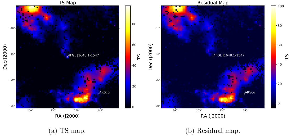
Figure 4.27: TS (a) and residual map (b) centred on 4FGL J1648.1-1547 (RA:252.027°, Dec:-15.793, J2000, Decimal Equatorial) for the 10-year period (4 August 2008 to 18 March 2019), including AR Sco (bottom right).
