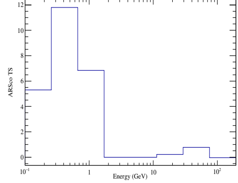
(b) TS values vs energy of \gamma -ray photons.
