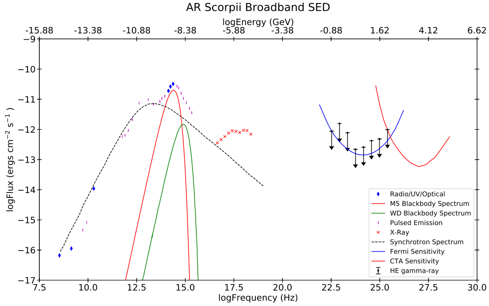
Figure 10: AR Sco broadband SED showing the gamma-ray upper limits in relation to the Fermi- LAT 10 year 1 (blue) and CTA-South 50 hour 2 (red) sensitivity curves.
