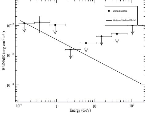
(a) Energy flux SED obtained using bdlikeSED .
