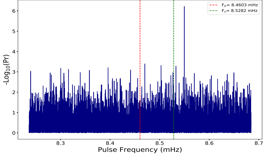
Figure B.1: 10-year (4 August 2008 - 18 March 2019) Rayleigh periodogram of AR Sco in the energy range of 100 MeV to 30 GeV, covering frequencies from 8.2 – 8.7 mHz. Additional line marker added showing the current model for the fundamental beat ( F_b = 8.4603 mHz) and spin ( F_s = 8.5282 mHz) frequency of the white dwarf in AR Sco. Periodogram produced using the ephemeris from Gaibor et al. (2020).
