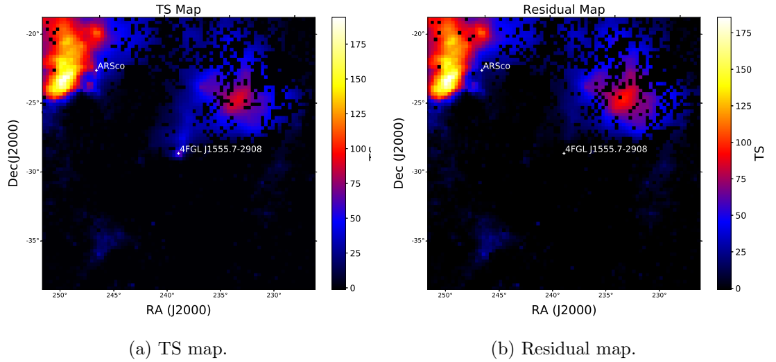
Figure 4.28: TS (a) and residual map (b) centred on 4FGL J1555.7-2908 (RA:238.921°, Dec:-29.137, J2000, Decimal Equatorial) for the 10-year period (4 August 2008 to 18 March 2019), including AR Sco (top left).
