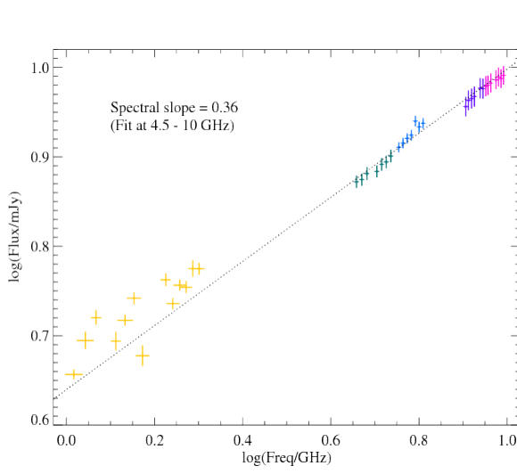
Figure 2.8: Radio SED of AR Sco, averaged over a full orbital period ( P_o = 3.56 h). The dashed line indicates a spectral fit of the form F_\nu \propto \nu^\alpha , fitted to the data in the 5 GHz and 9 GHz bands, extrapolated to the 1.5 GHz band. The best fit is found at \alpha = 0.358 \pm 0.015 . Adopted from Stanway et al. (2018).
