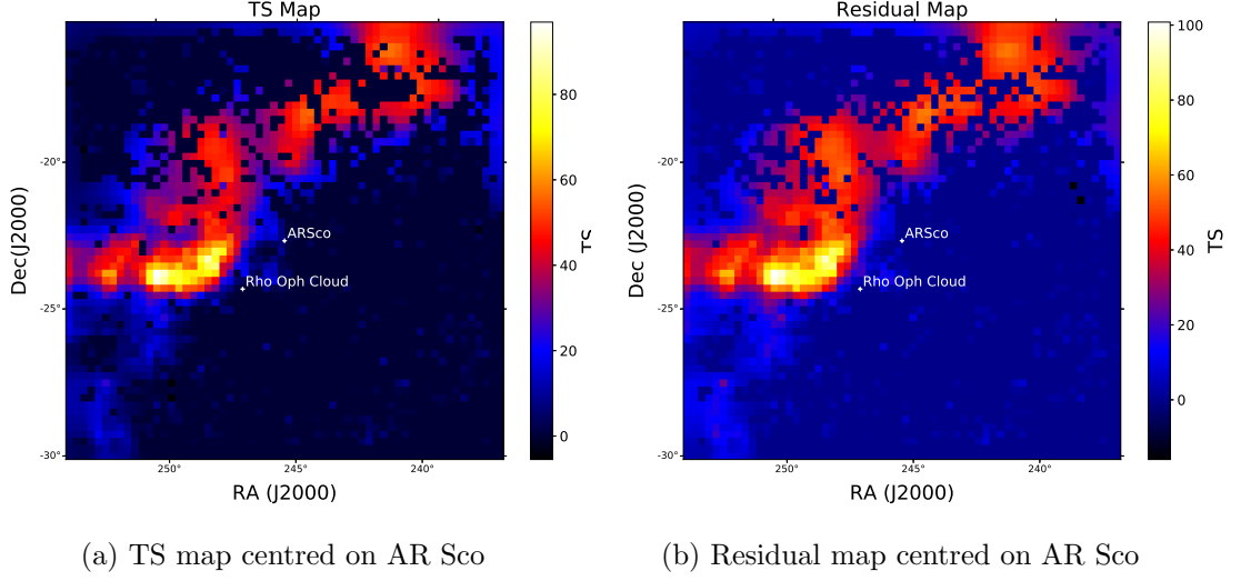
Figure 4.7: Plots of AR Sco’s TS values within its ROI where (a) shows the TS map centred on AR Sco and (b) shows the residual map centred on AR Sco. By comparing these two maps very low emission excess (a few bright pixels) can be seen at the coordinates centred on AR Sco in (a) but not in (b).
