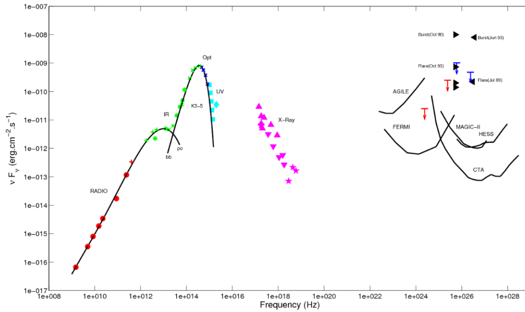
Figure 2.16: The spectral energy distribution of AE Aqr, with sensitivity curves of gamma-ray satellites and ground based telescopes. [16]
