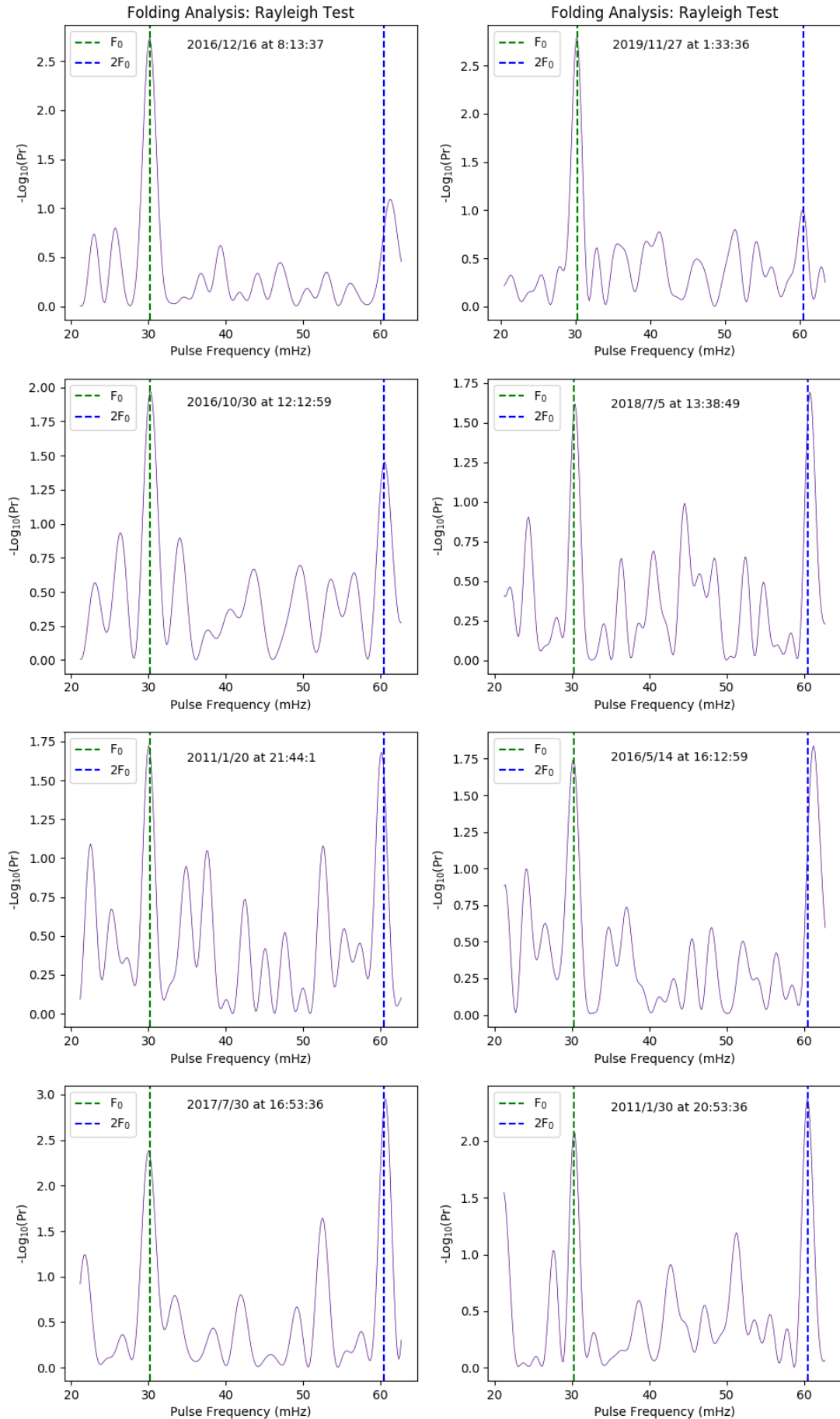
Figure B.23: The pulse profiles of AE Aqr showing the pulses at or near the fundamental frequency and the first harmonic.
