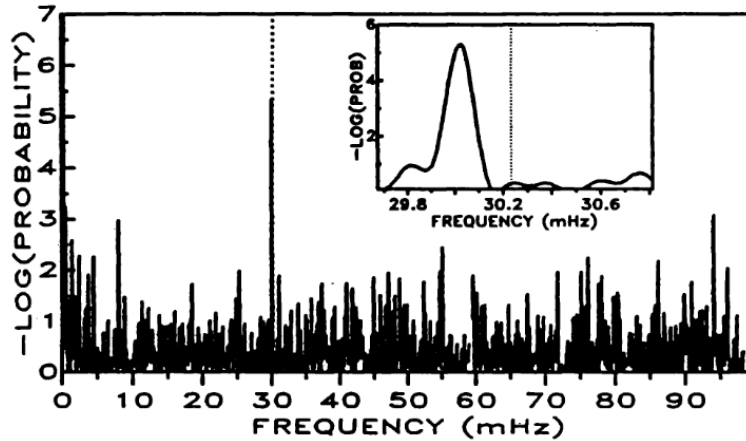
Figure 2.12: The periodogram of the very high energy Tera electron volts (VHE-TeV) pulsed emission of AE Aqr. The dotted line represent the very stable white dwarf spin frequency of 30.23 mHz, where the insert shows the shifted p VHE-TeV periodic signal [11].
