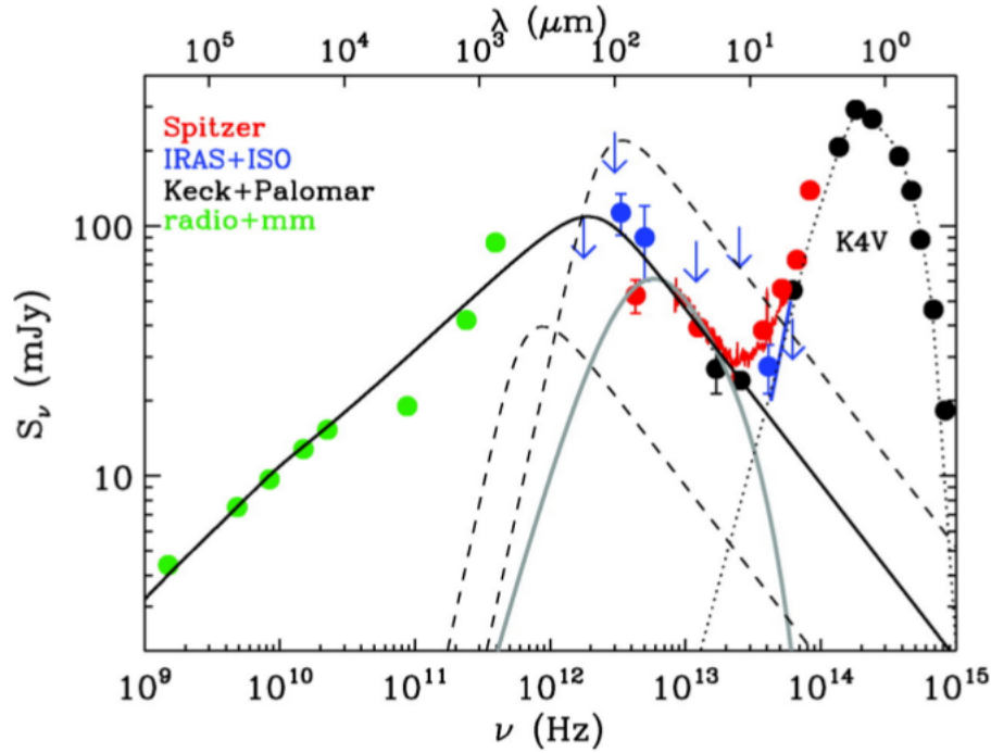
Figure 2.10: The spectral energy distribution of AE Aqr from radio to optical emission with proposed model behind the emission[9]
