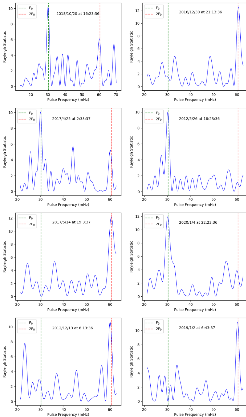
Figure B.22: The pulse profiles of AE Aqr showing the pulses at or near the fundamental frequency and the first harmonic.
