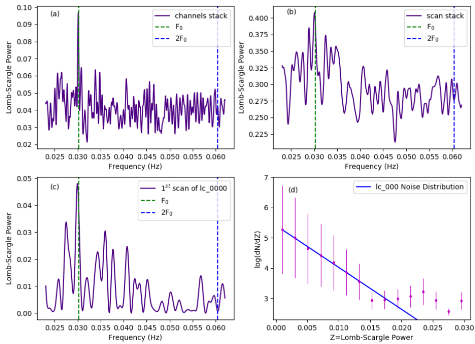
Figure 4.14: (a) Stacked lc_0000, lc_0001, lc_0002 power spectrum (b) stacked power spectrum for scans 1, 2, and 3 [all channels], (c) power spectrum corresponding to the lower channel of the first scan, and (d) the noise distribution of the 6 seconds binned data for the lower channel.
