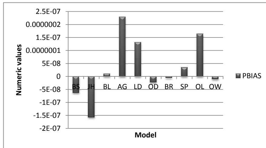
Figure 3. PBIAS for Dry season
