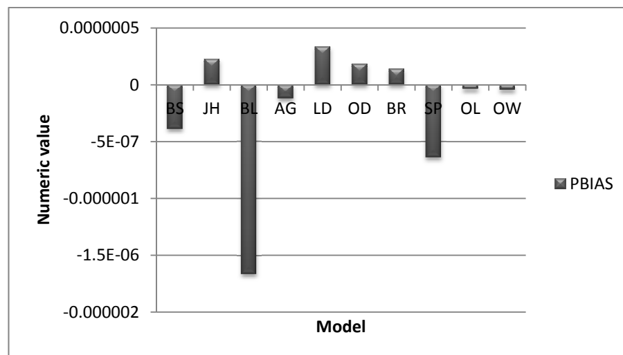
Figure 4. PBIAS for Rainy season
