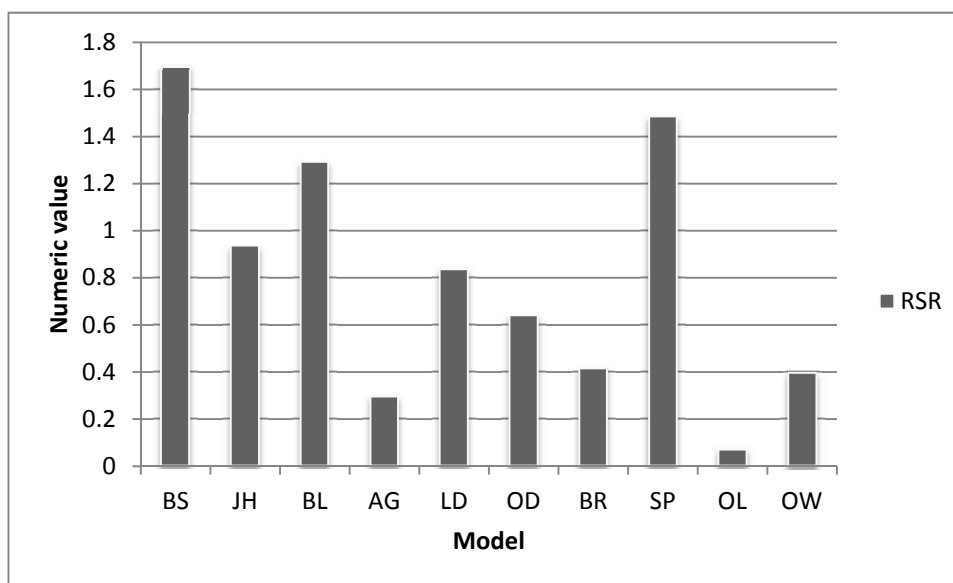
Figure 6. RSR for Rainy season
