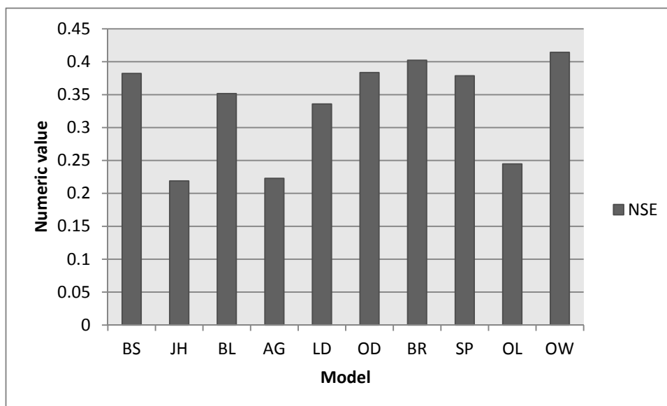
Figure 8. NSE for Rainy season
