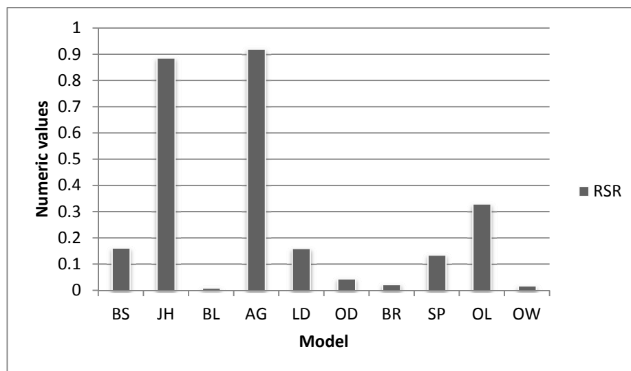
Figure 5. RSR for Dry season
