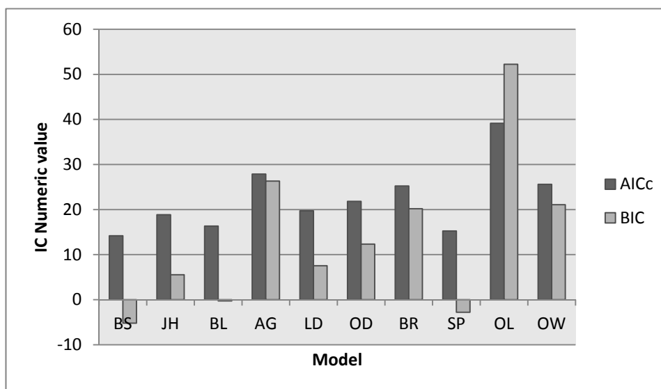
Figure 2. AICc and BIC values for Rainy season
