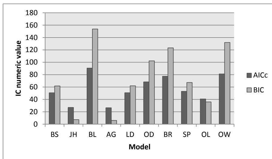
Figure 1. AICc and BIC values for Dry season
