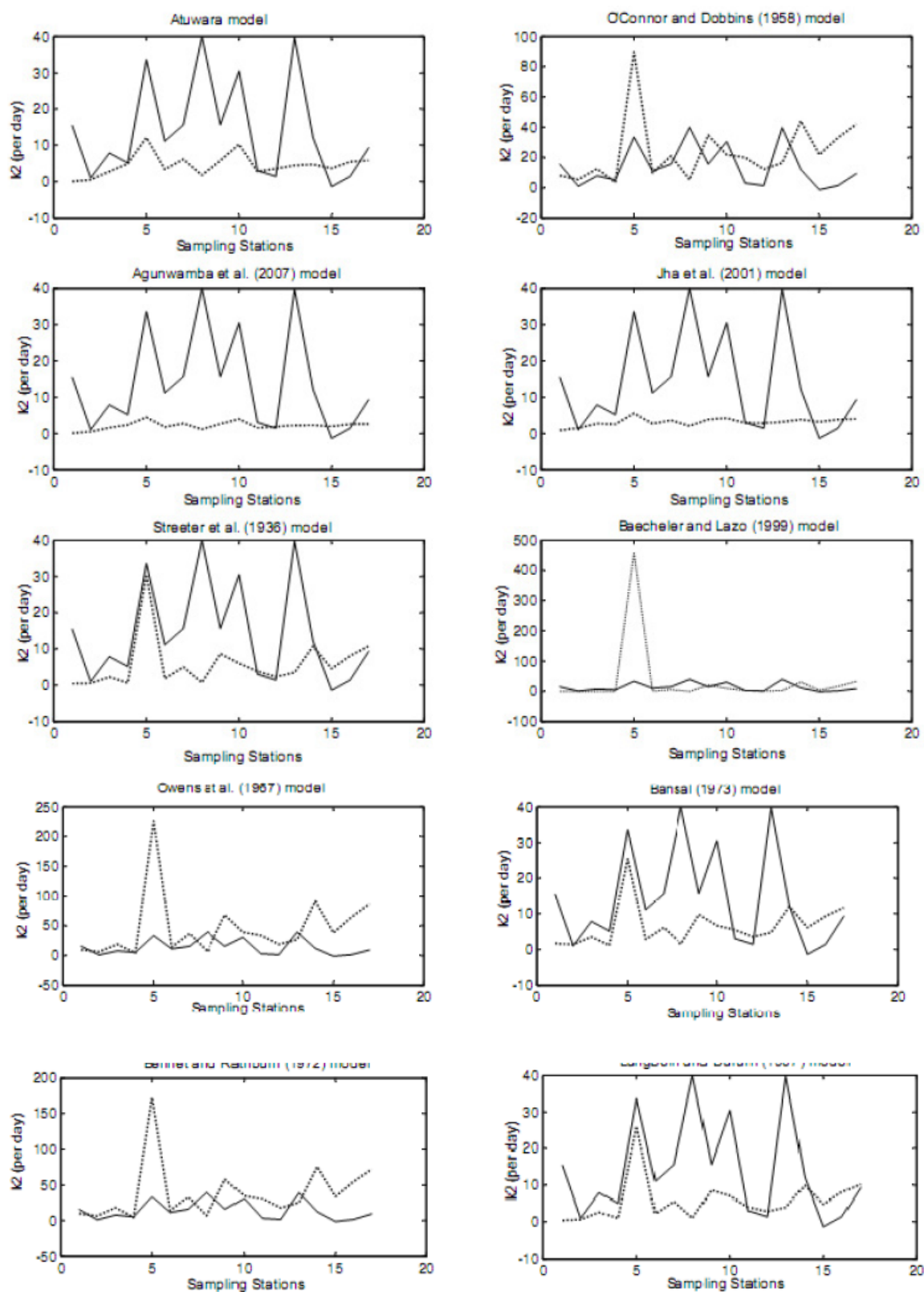
Figure 9. Plot of observed and simulated k_2 values for dry season (reproduced with permission from Omole and Longe, 2012)
