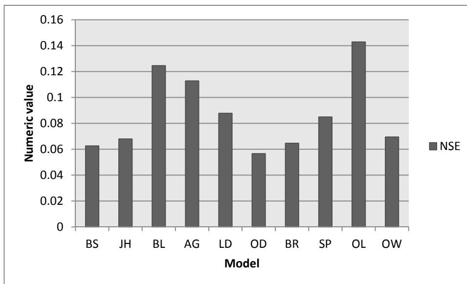
Figure 7. NSE for Dry season
