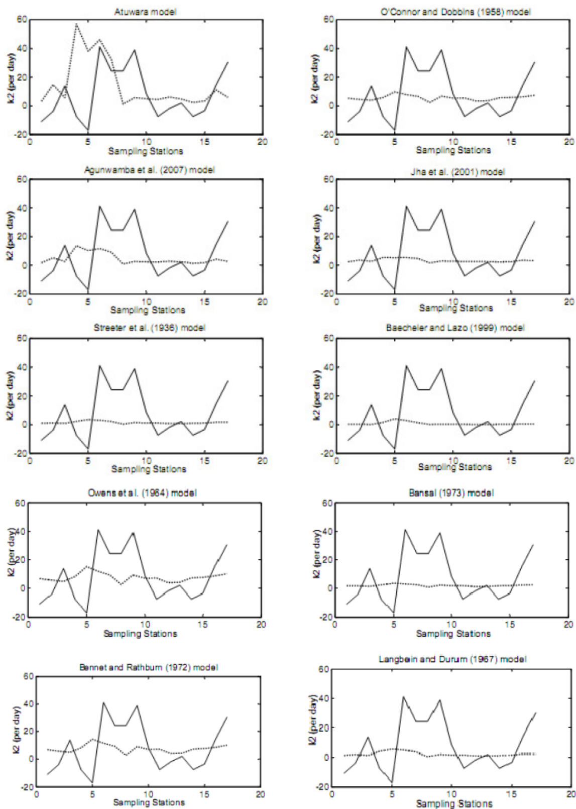
Figure 10. Plot of observed and simulated k_2 values for rainy season (reproduced with permission from Omole and Longe, 2012)
