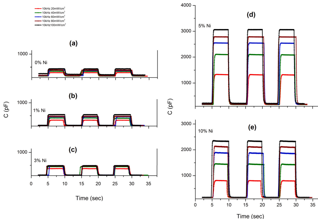
Fig. 12. Photo-capacitance responses of the diodes to 10 kHz, 50% duty-cycle illumination for varying Ni concentrations of 0, 1, 3, 5 and 10% in (a), (b), (c), (d) and (e), respectively.
