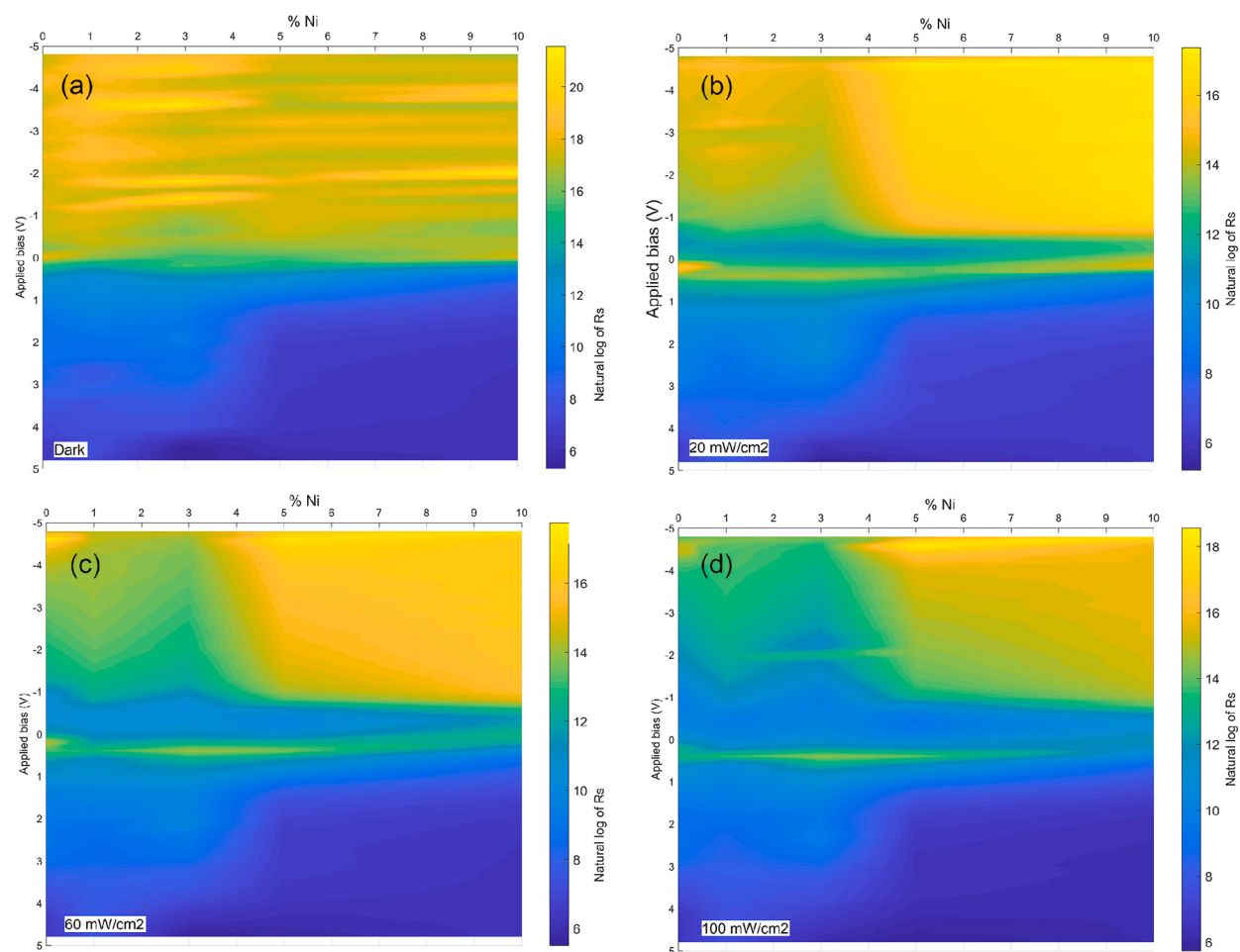
Fig. 3. Color map representation of \ln R_s(k) versus applied bias, %Ni content, and illumination. The illumination intensities are 0, 20, 60 and 100 mW/cm 2 in (a), (b), (c), and (d), respectively.
