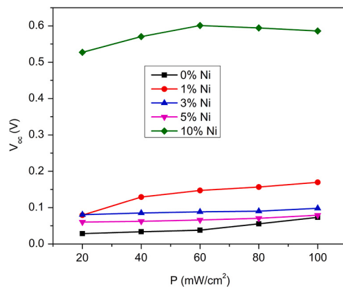
Fig. 10. R_s -corrected open-circuit voltages, V_{oc} , for various %Ni content in the fabricated diodes.
