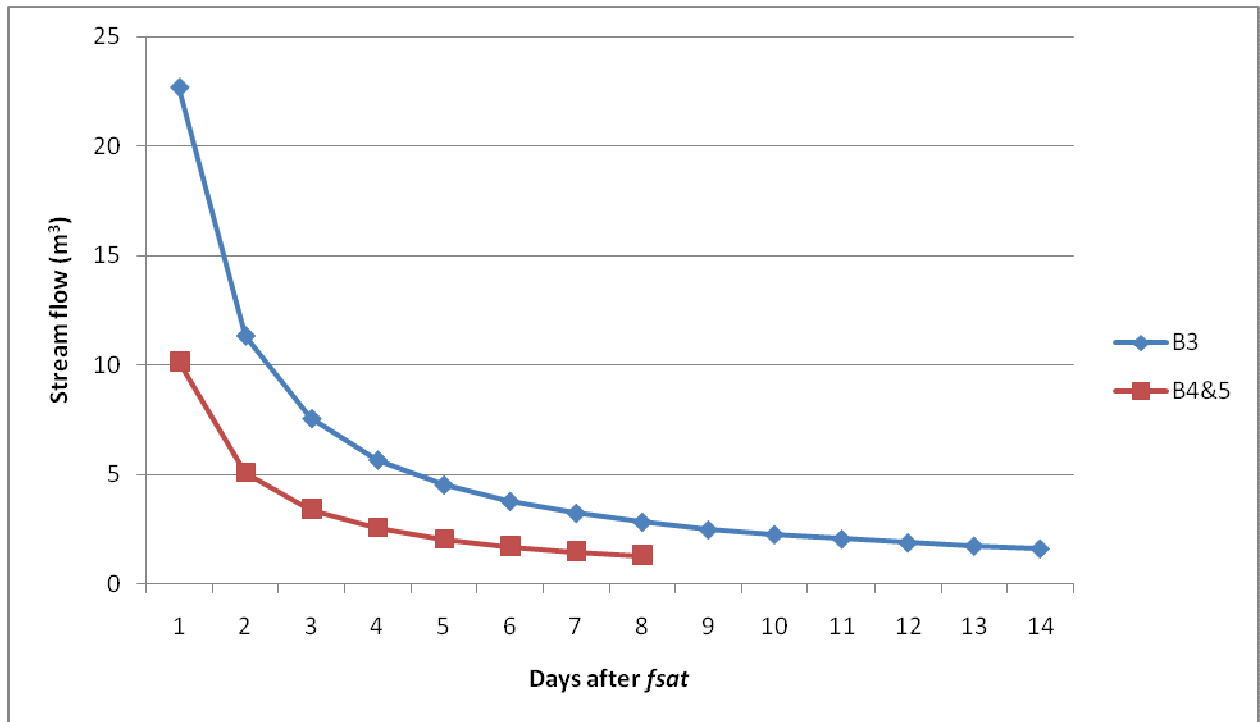
Figure 5.15 Estimated streamflow ( \text{m}^3 ), all of it originating from interflow, i.e. interflow water only, from catchments B3 and B4&5 in days after f_{sat} based on the drainage equations presented in Table 5.28.
