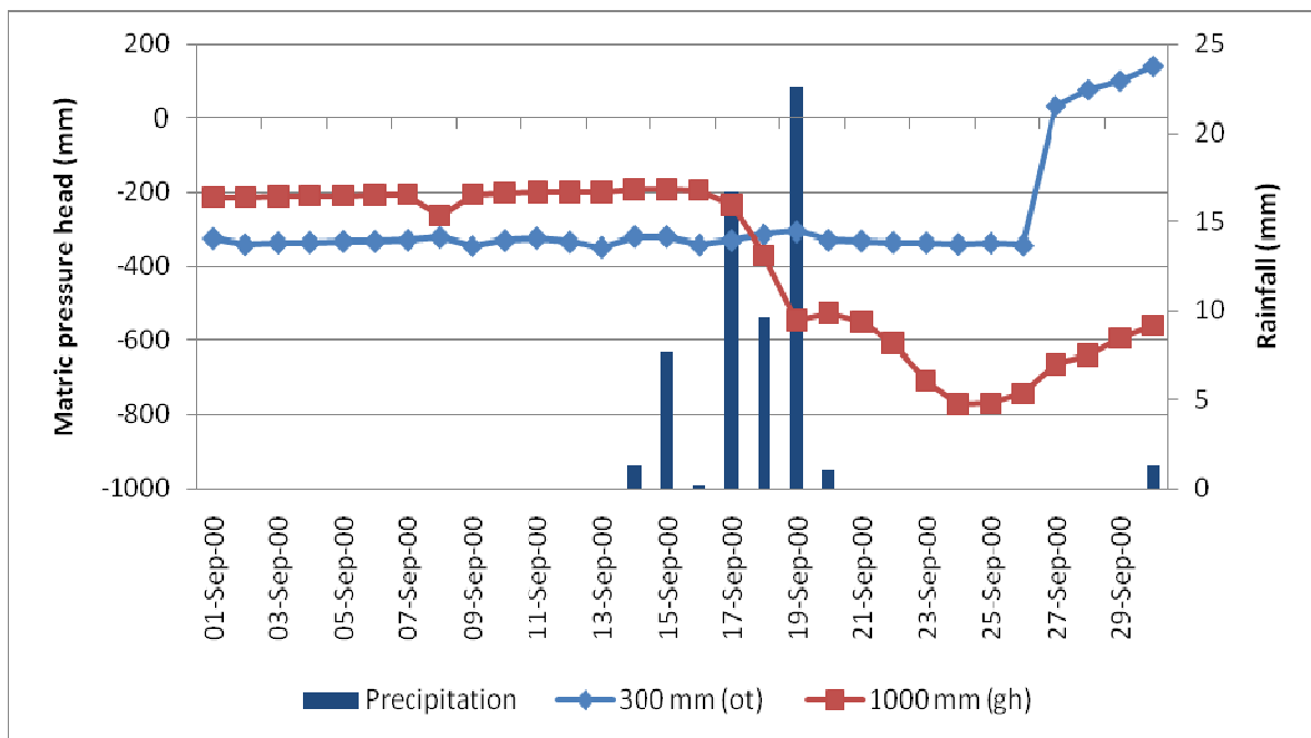
Figure 4.19 Matric pressure head (mm) vs. rainfall (mm) at different depths for the Ka1000 at Uc4 during period 1, describing the reaction of a responsive soil near the toeslope of the catchment following a dry period.
