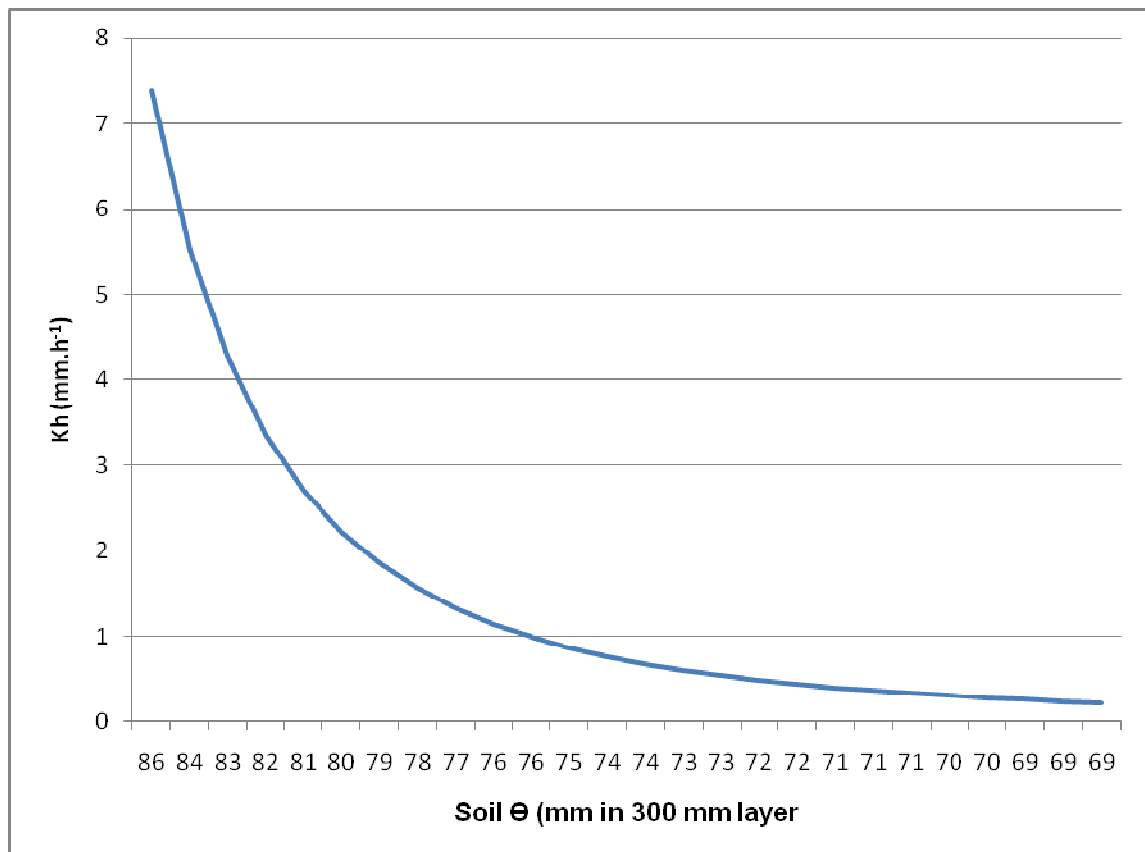
Figure 4.27 \Delta K(h) ( \text{mm} \cdot \text{h}^{-1} ) with \Delta \Theta (mm in 300 mm layer) based on equation 4.4.
