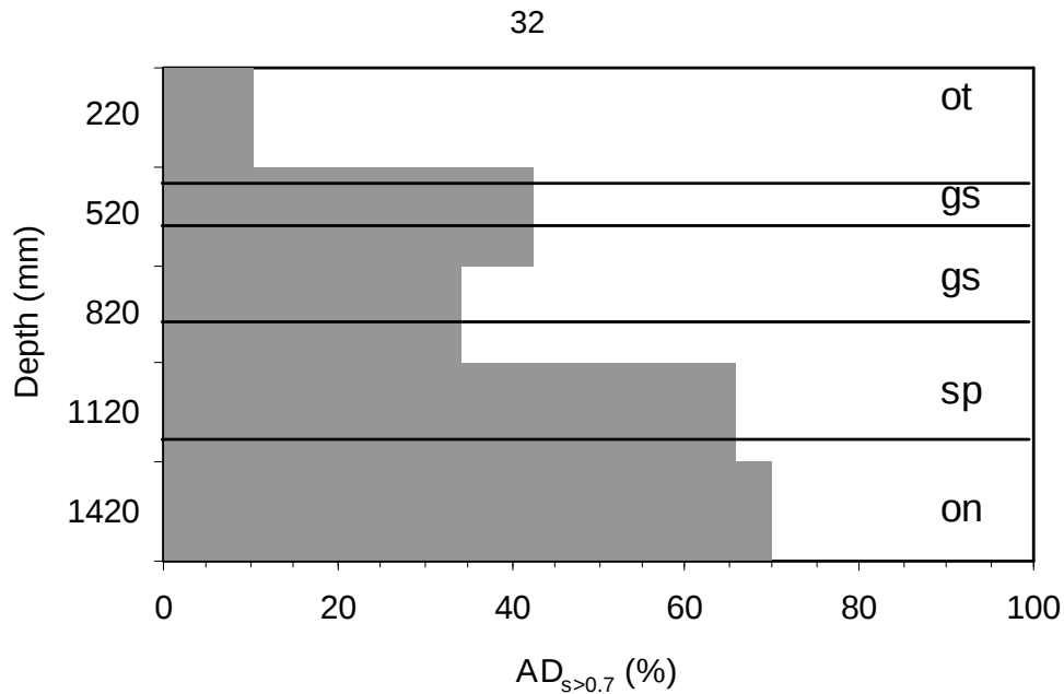
Figure 3.3 Mean AD_{s>0.7} (%) values in a typical interflow soil P225, Longlands 1000, Weatherley (Van Huyssteen et al. , 2005).
