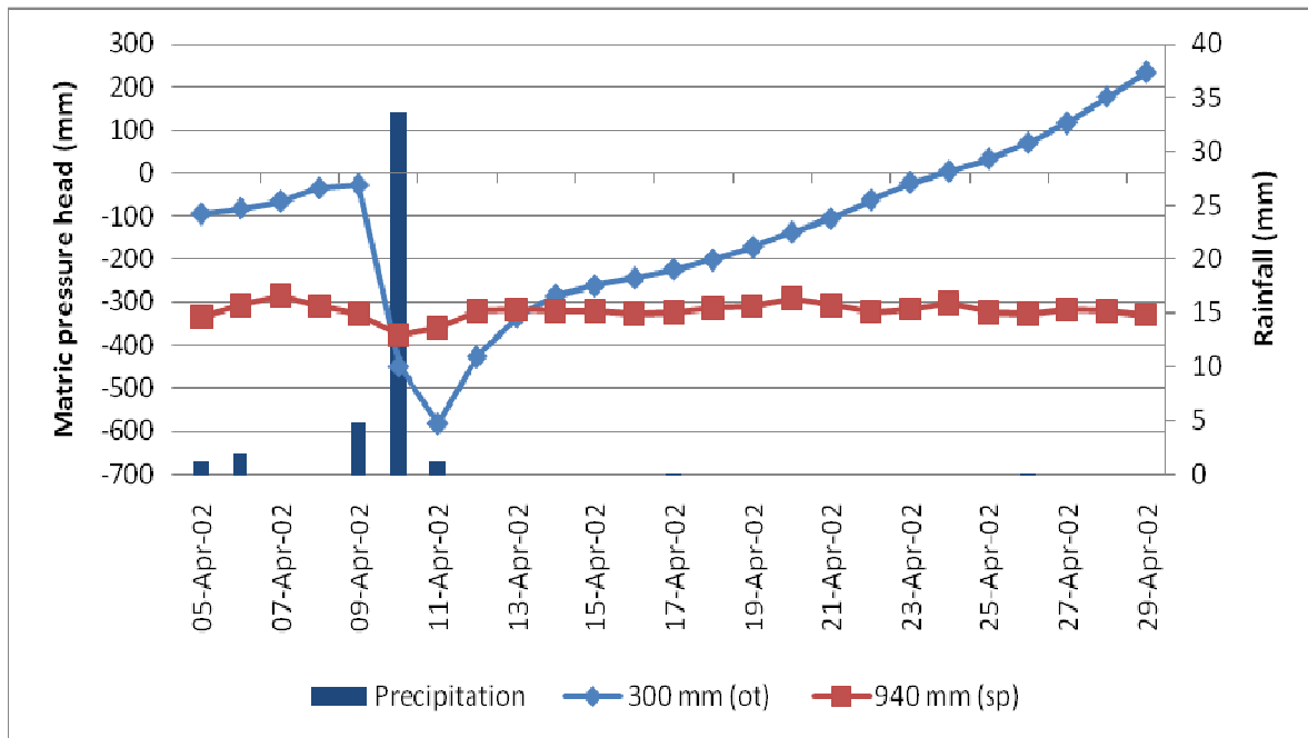
Figure 4.11 Matric pressure head (mm) vs. rainfall (mm) at different depths for the Bd1100 at Uc8 during period 4, describing the response of an interflow soil near the Molteno rock outcrop of the catchment following a wet period.
