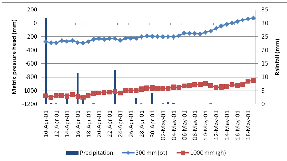
Figure 4.20 Matric pressure head (mm) vs. rainfall (mm) at different depths for the Ka1000 at Uc4 during period 3, describing the reaction of a responsive soil near at the toeslope of the catchment following a wet period.
