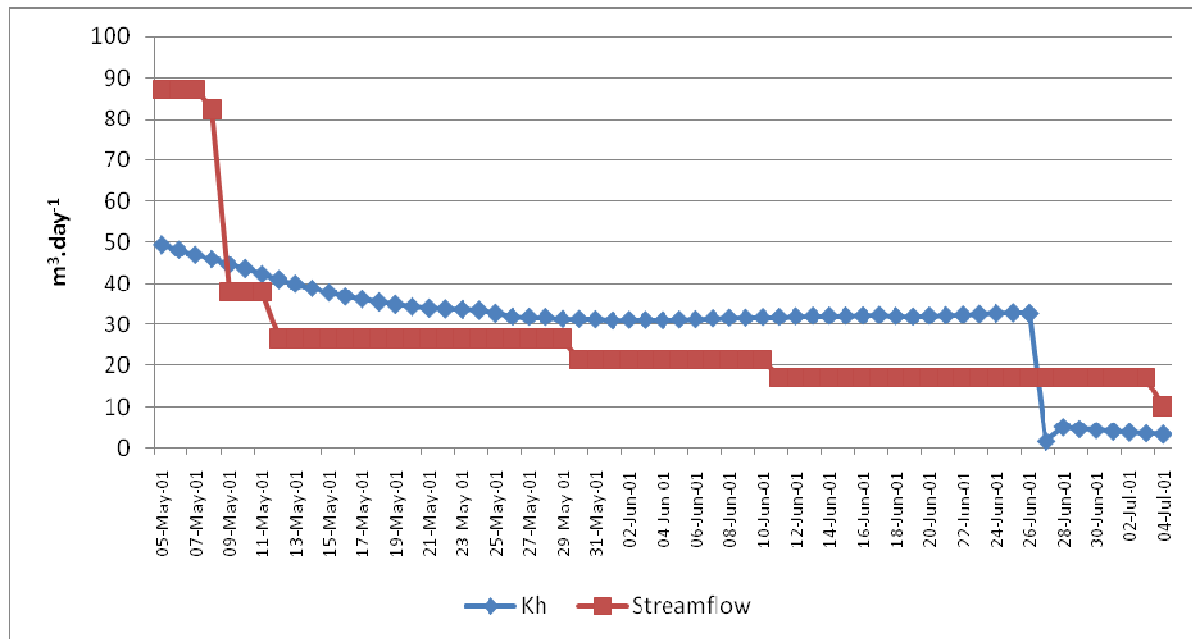
Figure 4.28 \Delta K(h) (m 3 .day -1 ) vs. streamflow (m 3 .day -1 ) for 60 day period starting 5 May 2001.
