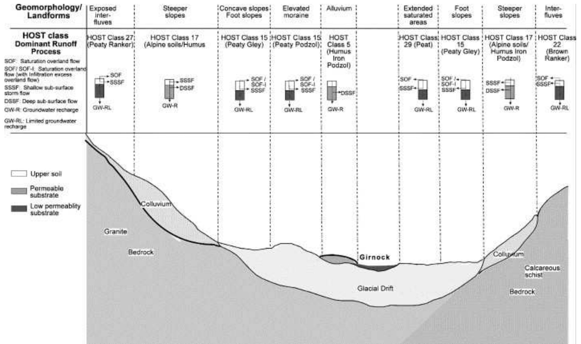
Figure 6.1 Conceptual model of the distribution of soil hydrological properties according to HOST in the Girnock (Soulsby et al. , 2007).
