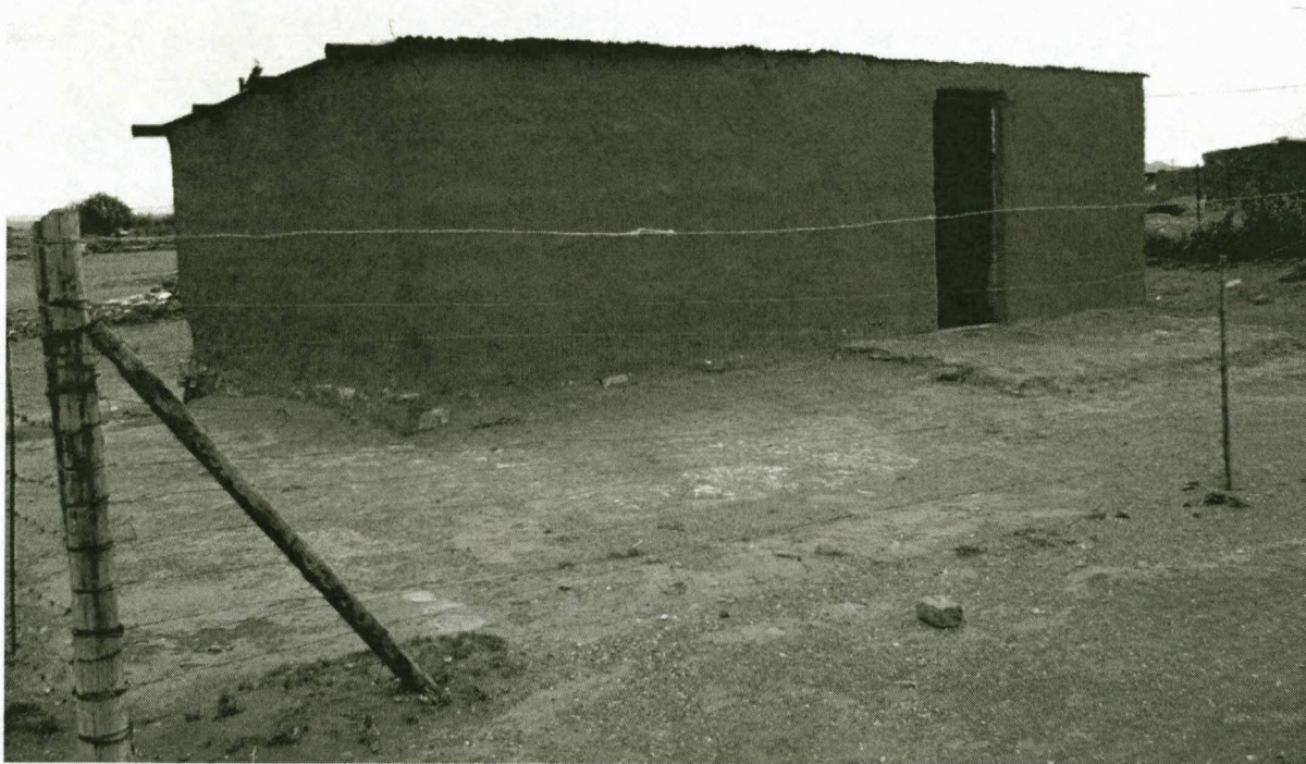
Figure 4.16: A well maintained adobe dwelling with plinth of available rubble and slightly raised threshold for preventing storm water from entering dwelling
