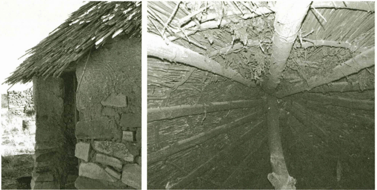
Figure 4.19: Detail of rondavel: Remnants of dagha plastering on the external facade (left) and central post supporting the fluitjiesriet roof (right)
