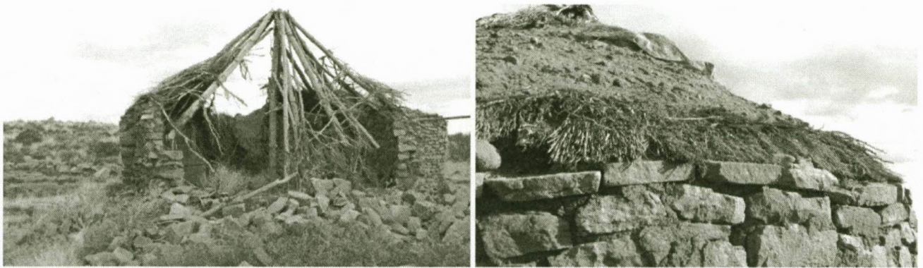
Figure 4.22: Thick, coarsely laid stone walls and centre post providing structural integrity to the rondavel (left), and earth and on top of hessian bags on roof limiting earth from seeping into rondavel
