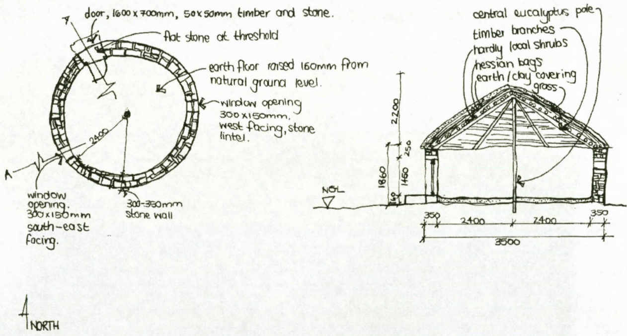
Figure 4.23: Sketches illustrating the method of construction used for the R391 rondavel
