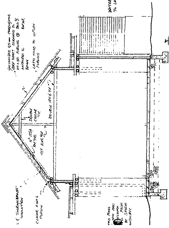
section b 1:50
