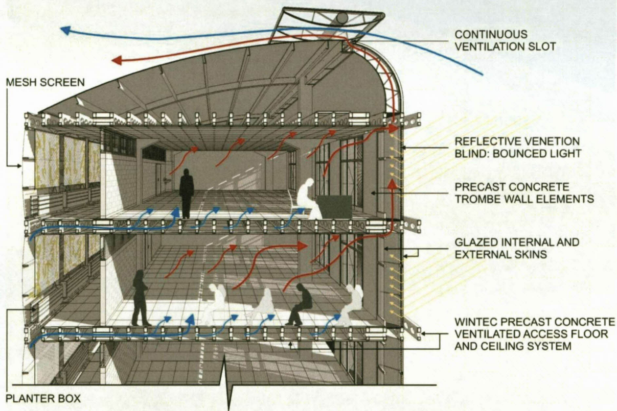
Figure 4.36: Section through New Auditoria and Teaching Complex illustrating the ventilation paths, trombe wall elements and Wintec precast concrete systems (Source: Stratford)
