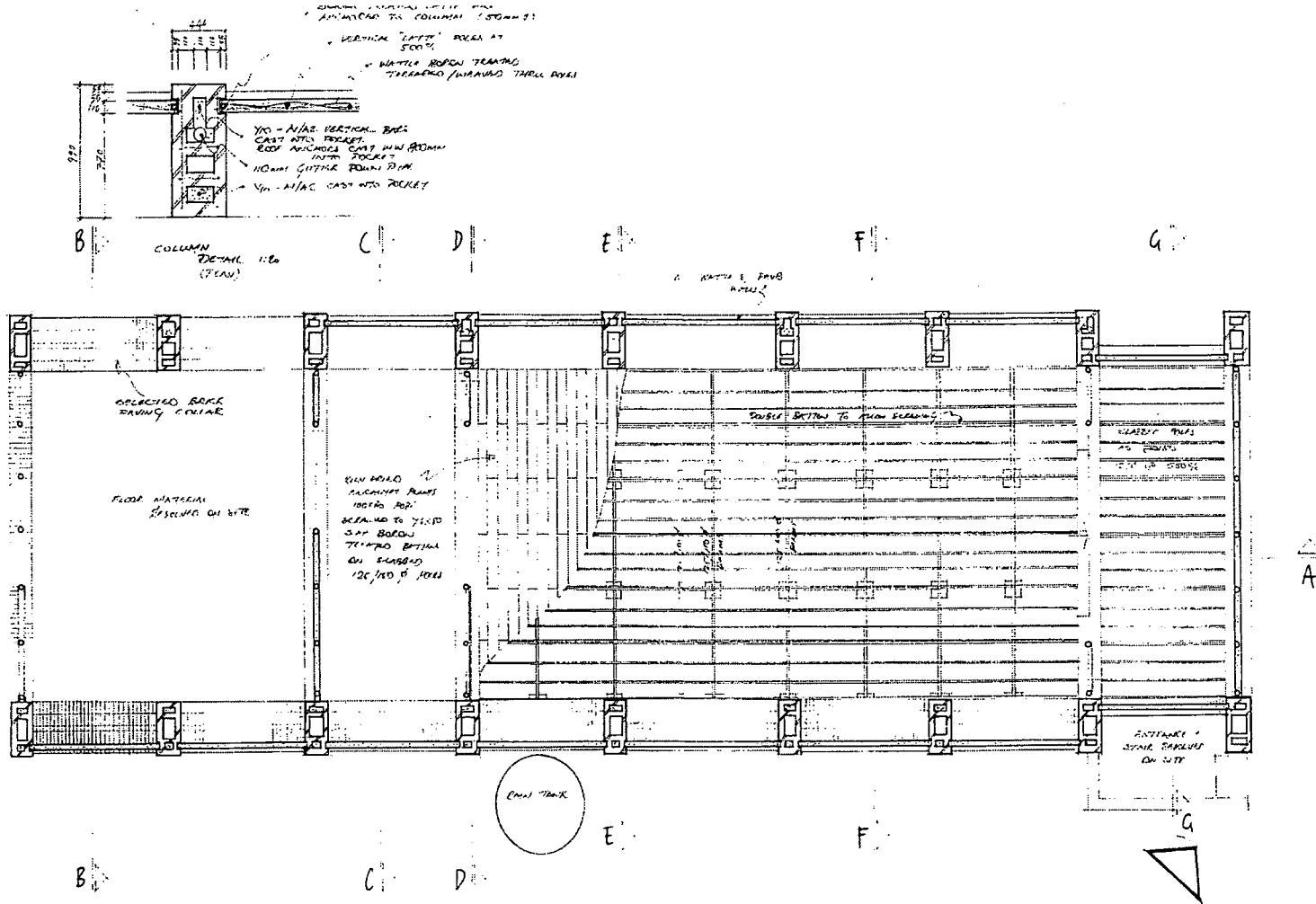
Floor structure plan 1:50
