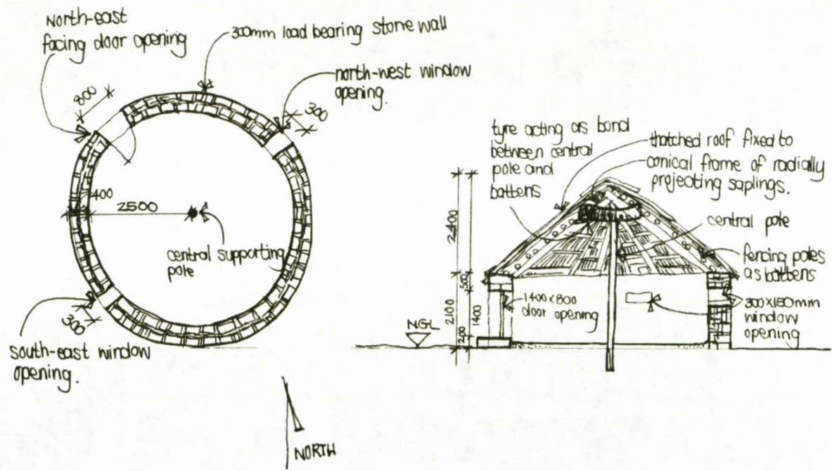
Figure 4.26: Illustration of the plan and section showing the structural detailing of the rondavel
