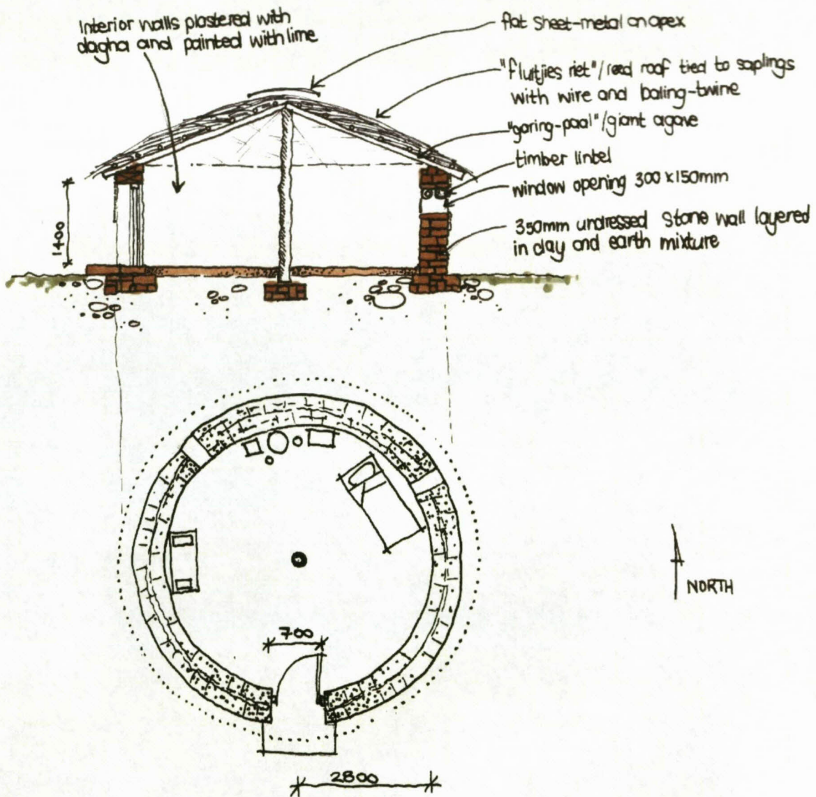
Figure 4.20: Section and plan illustrating the construction and spatial layout of the rondavel on the R390 between Hofmeyr and Steynsburg
