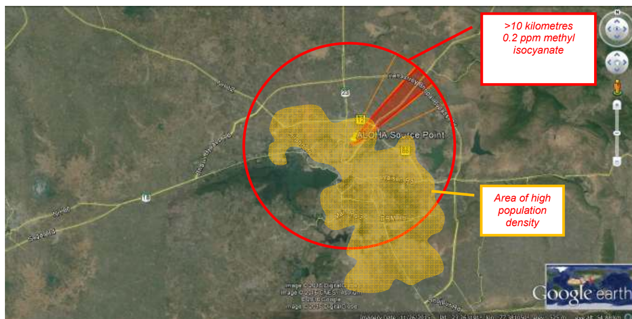
Figure 4.1 Surface area around the Union Carbide plant in Bhopal affected by the uncontrolled release of methyl isocyanate (Software source: ALOHA with own calculations)
