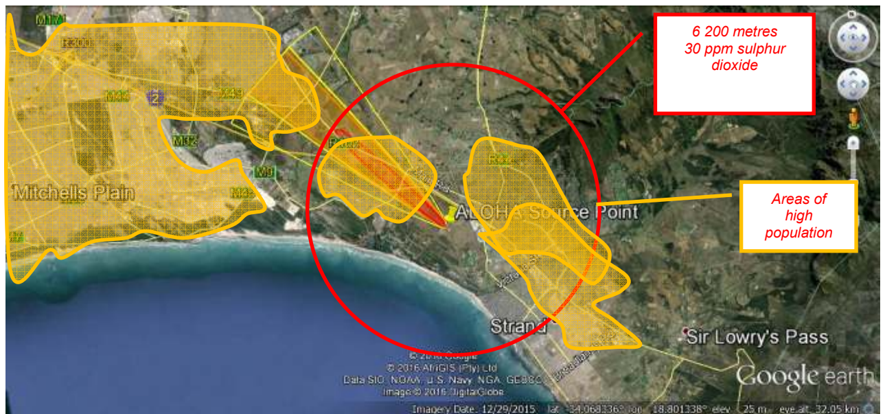
Figure 4.2 Surface area around the AECL sulphur stockpile in Somerset West affected by the uncontrolled release of sulphur dioxide (Software source: ALOHA with calculations by author)
