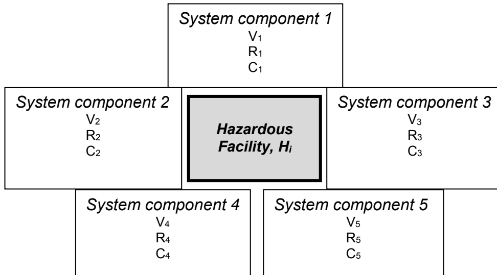
Figure 2.18 Vulnerability (V) of a system as a function of resilience (R) and coping capacity (C) of its discrete components (Source: Author)
